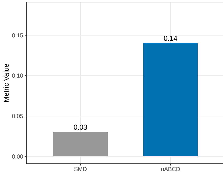
B) Metric comparison
