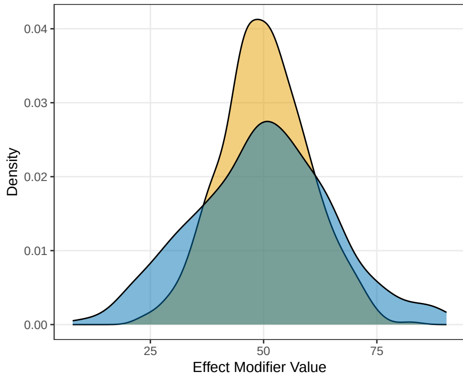
A) Same mean, different variance
