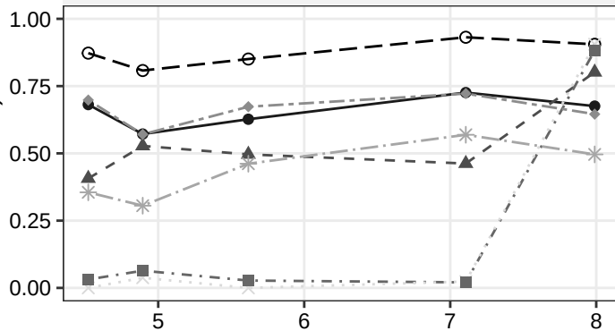
Set 3: Mixture world (moment-matched)
