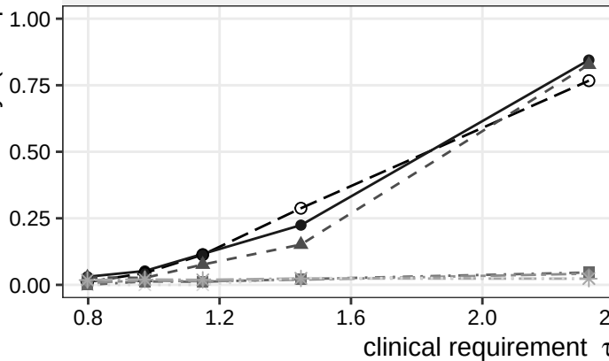
Set 3: Mixture world (moment-matched)
