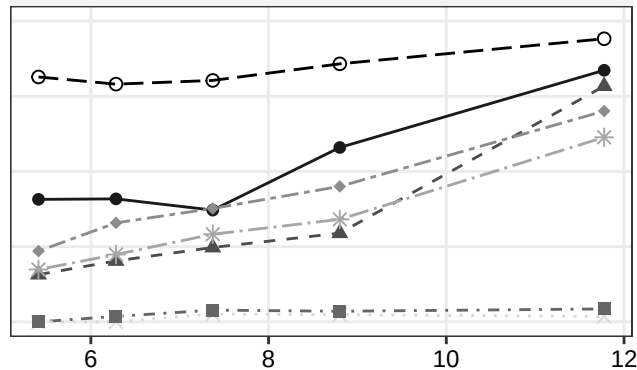
Set 4: Extremes world (rare displaced mass)
