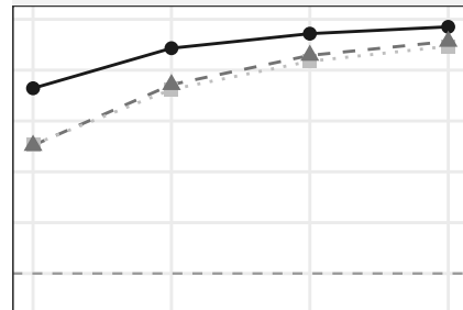
Set 2: Log-normal world Combined
