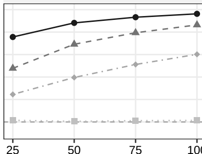
Set 2: Log-normal world Shape/dispersion
