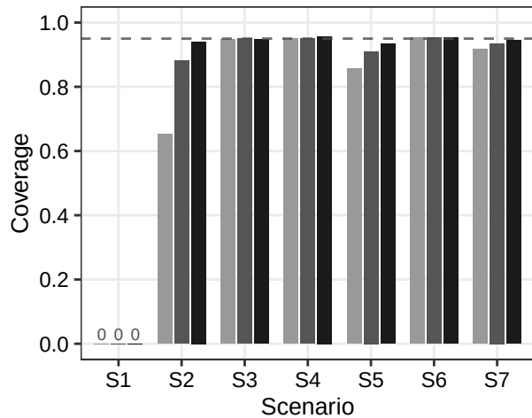
(B) Coverage
