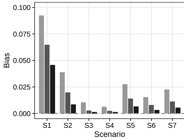
(A) Bias
