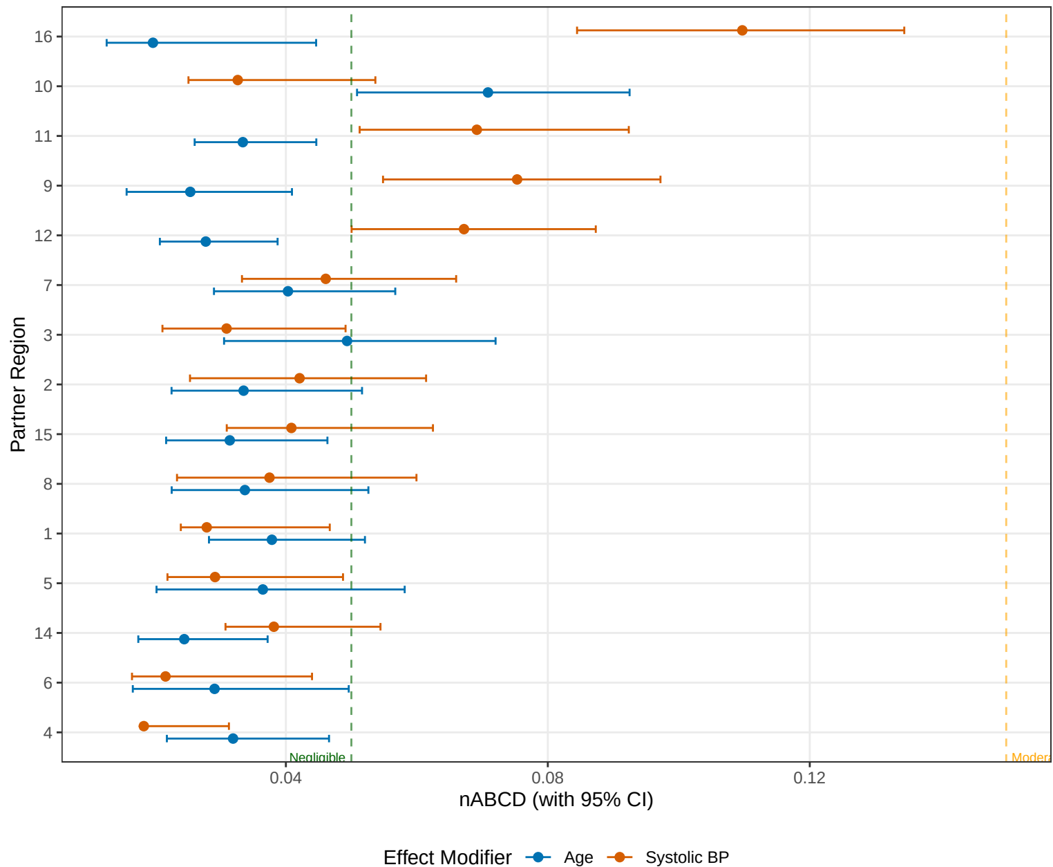
GUSTO-I: Bootstrap 95% CI for nABCD (Anchor = Region 13)
