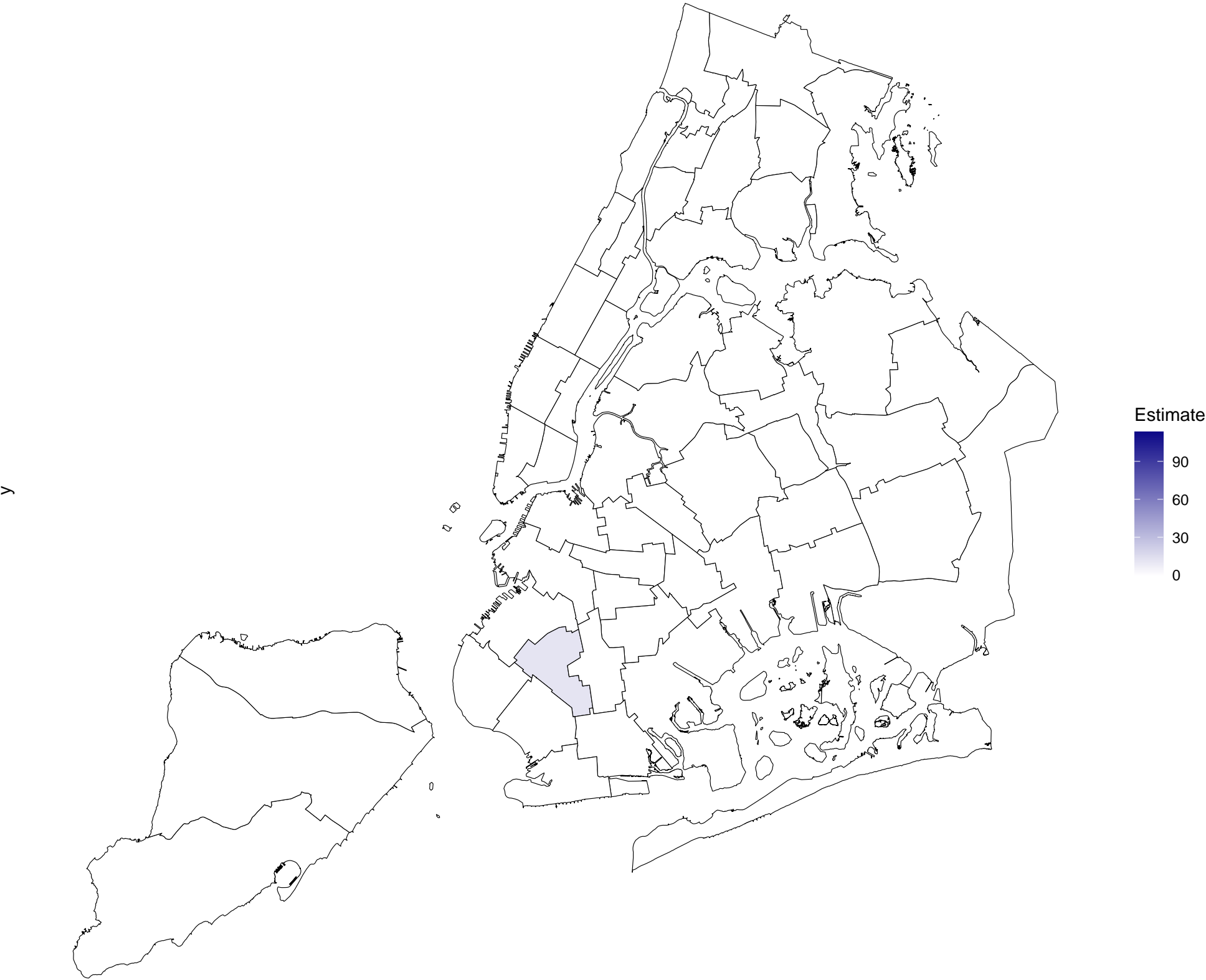
x Data table: B16001 Estimate of Language Spoken at Home; Polygon = PUMA ( \geq 100,000 pop.)
