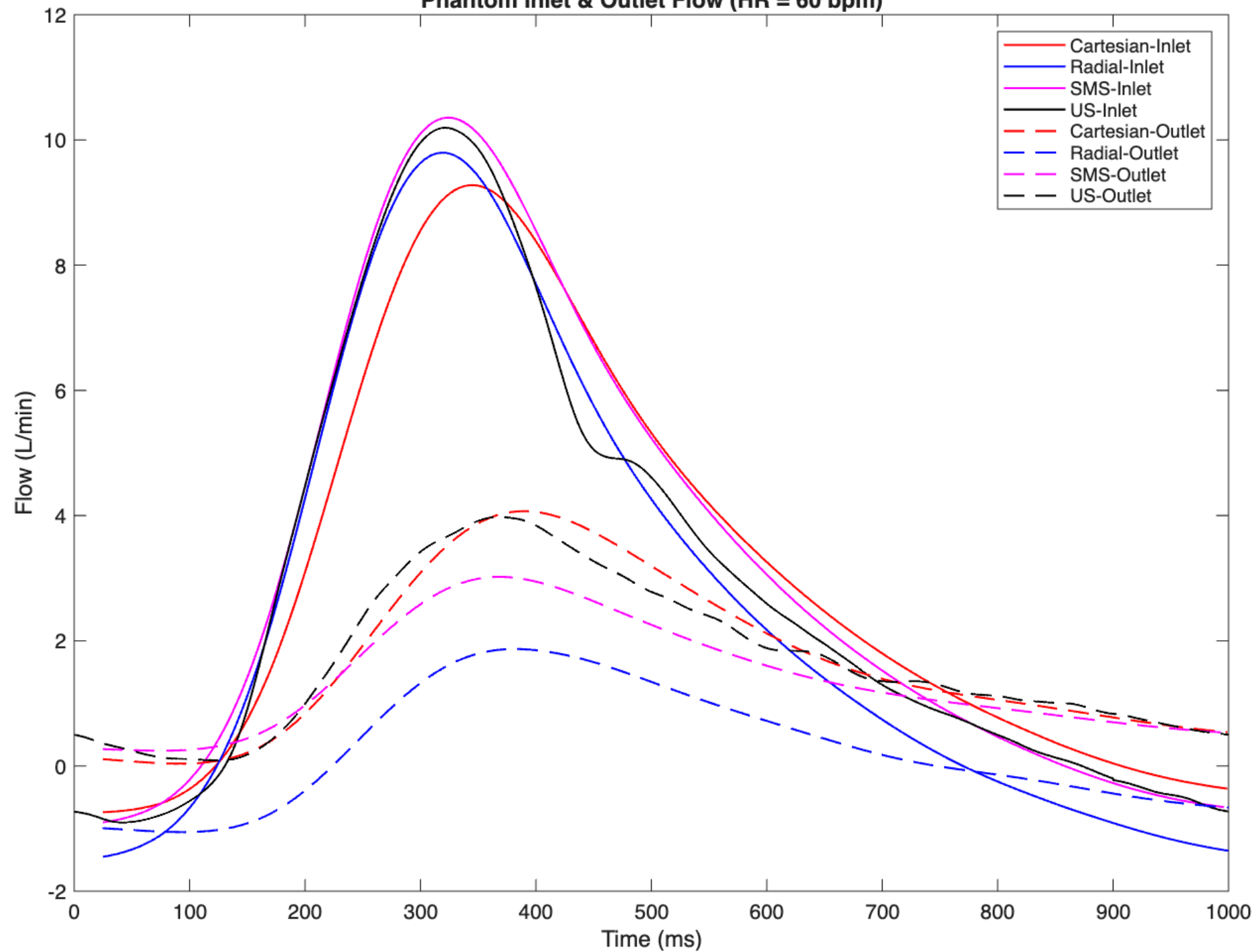
Phantom Inlet & Outlet Flow (HR = 60 bpm)
