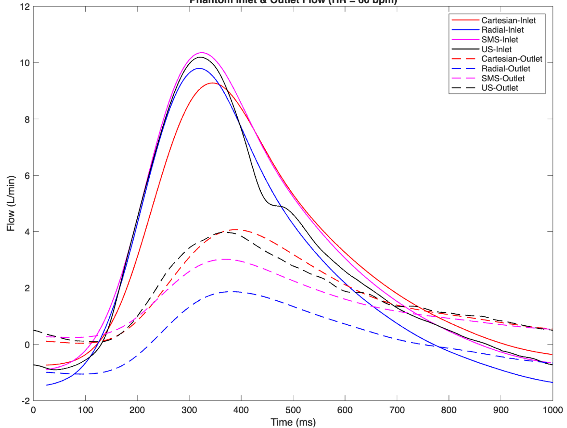
Phantom Inlet &amp; Outlet Flow (HR = 60 bpm)
