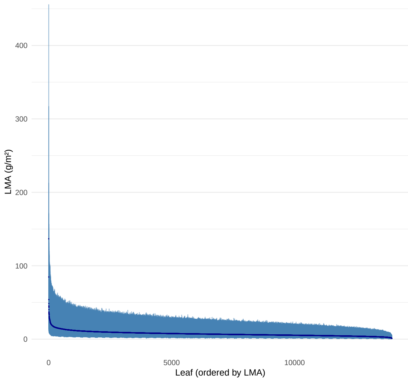
LMA Estimates with 95% Confidence Intervals
