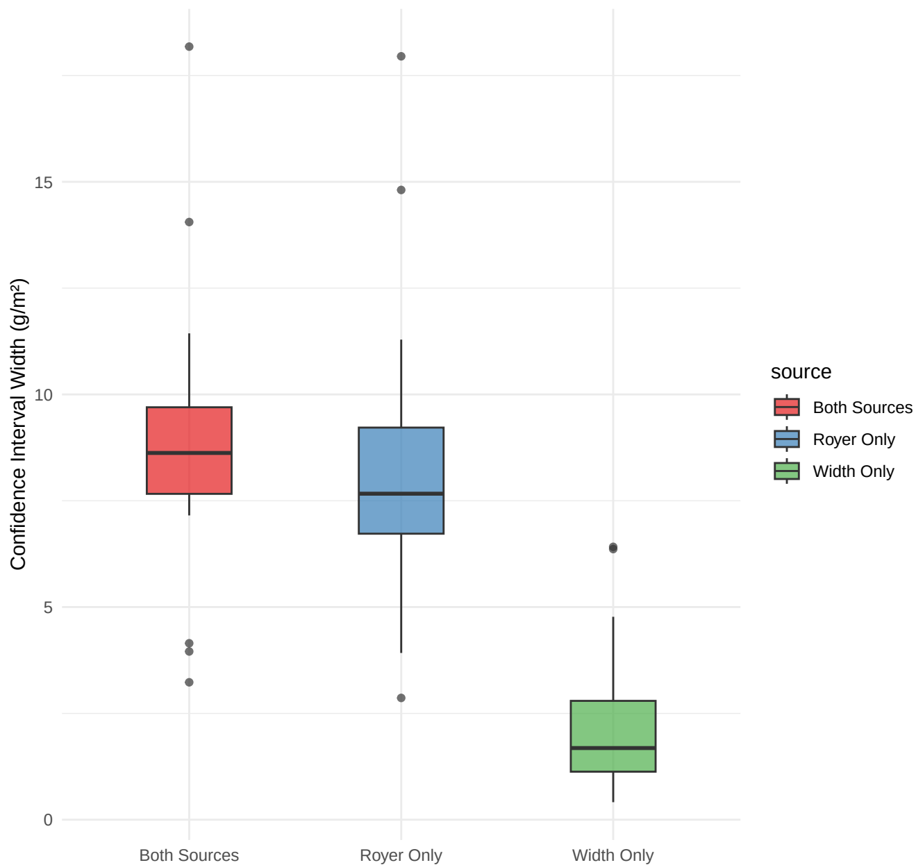
95% CI Width by Error Source
