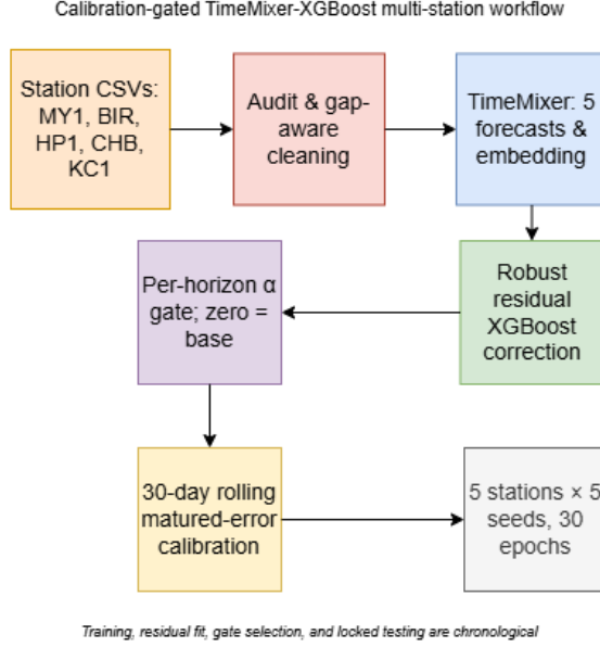
Fig. 1: End-to-end framework: TimeMixer generates base forecasts, and a later calibration interval fits and gates residual XGBoost before locked testing. separates neural validation, residual fitting, gate selection, and locked testing into distinct chronological eras.
