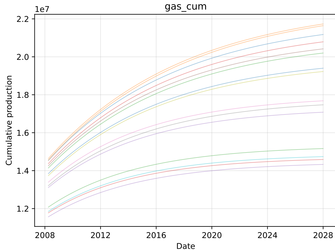
GP: Conditional 2028 Forecasts (Val Cases 71-85)
