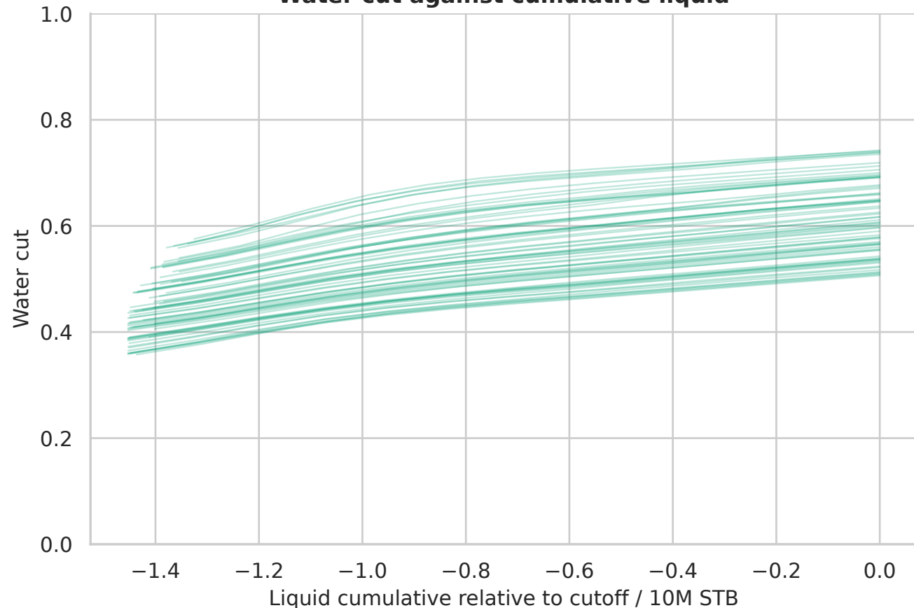
Water cut against cumulative liquid
