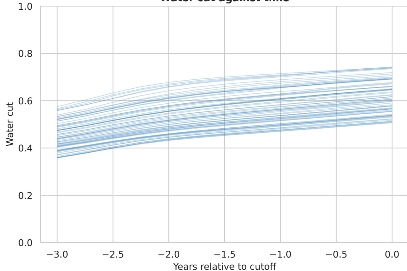
Water cut against time
