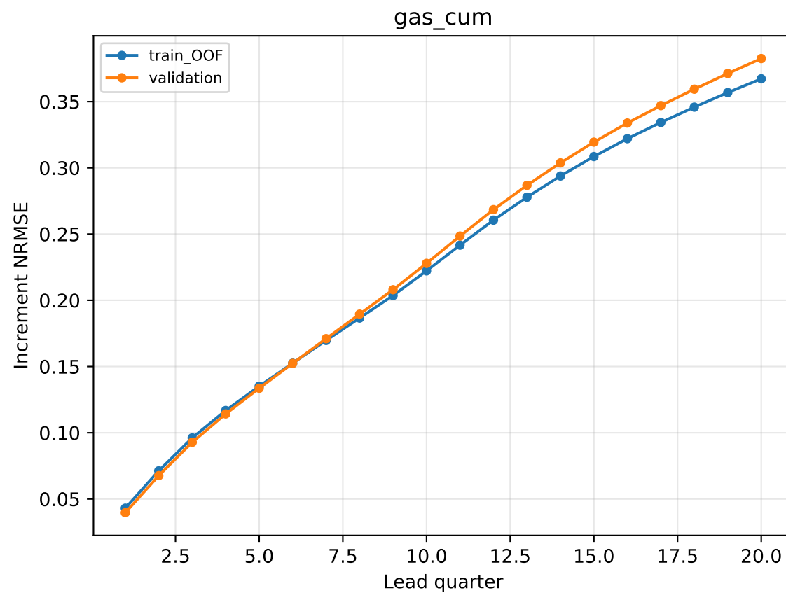
GP: 2003→5yr Error by Lead Quarter
