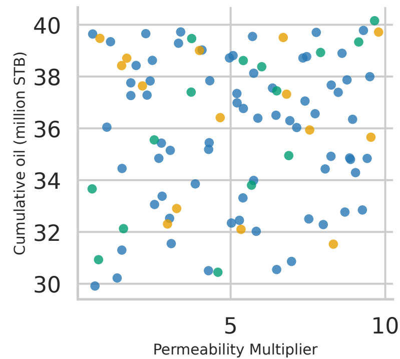
Uncertainty inputs versus cumulative production at 2008-01-01
