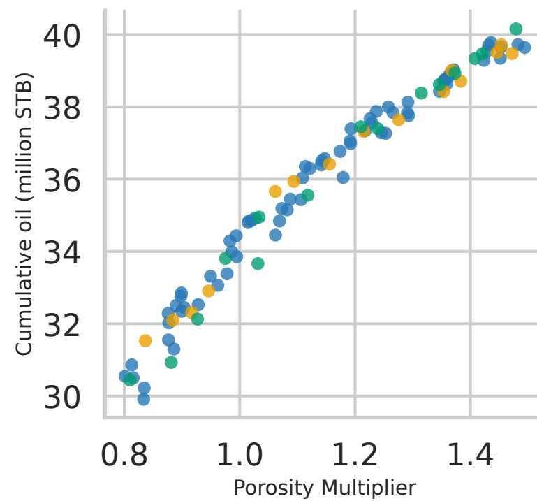
Uncertainty inputs versus cumulative production at 2008-01-01
