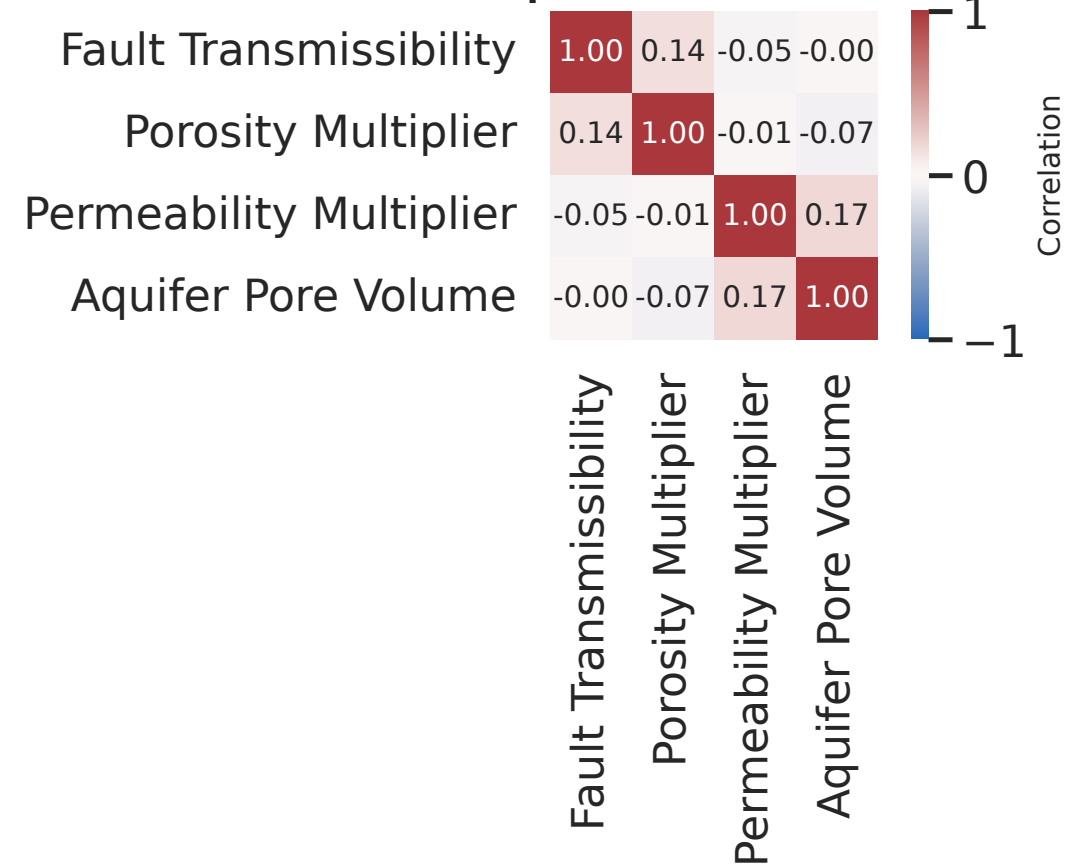
Spearman correlation
