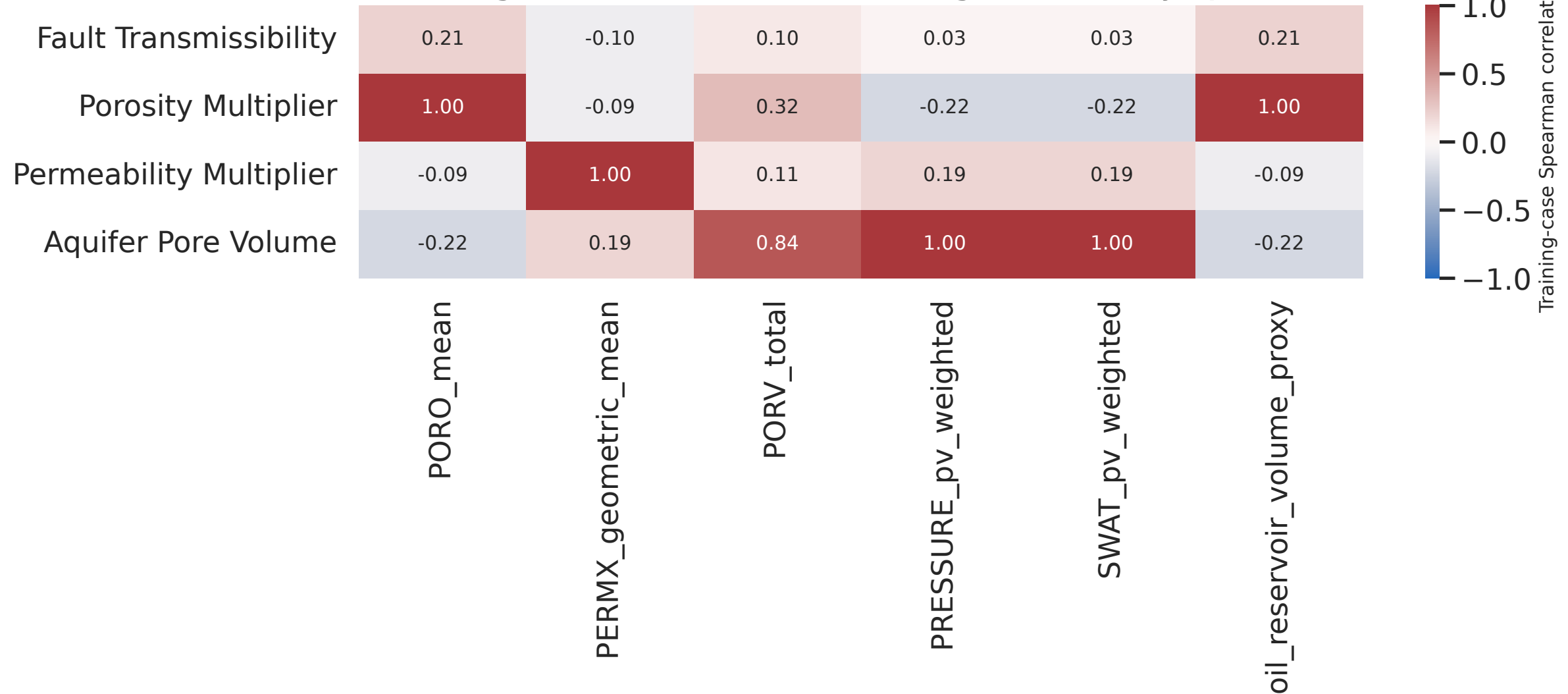
Are grid summaries alternative encodings of uncertainty inputs?
