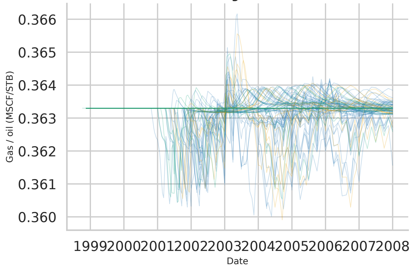
Produced gas-oil ratio
