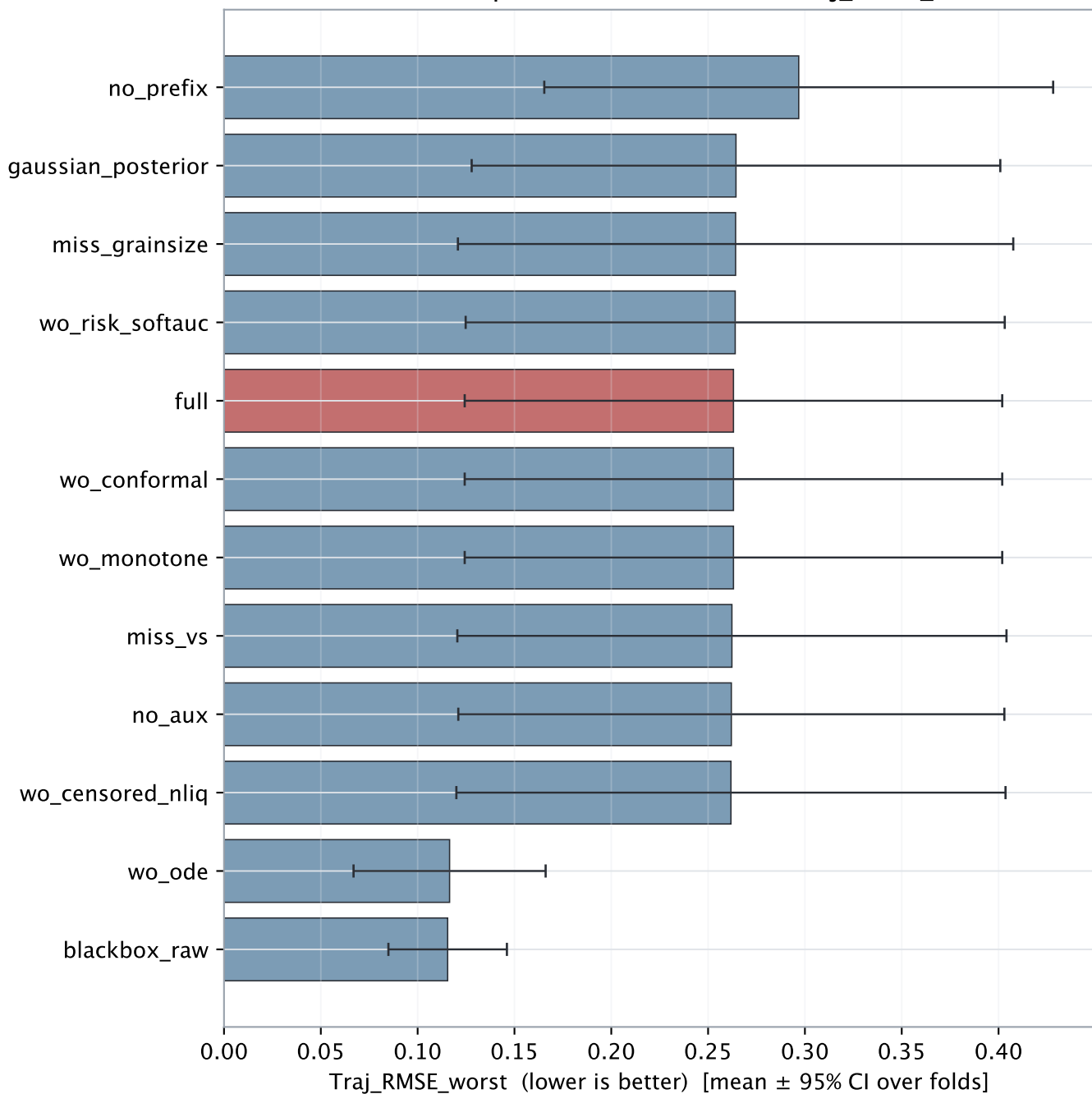
Ablation: component contribution to Traj_RMSE_worst
