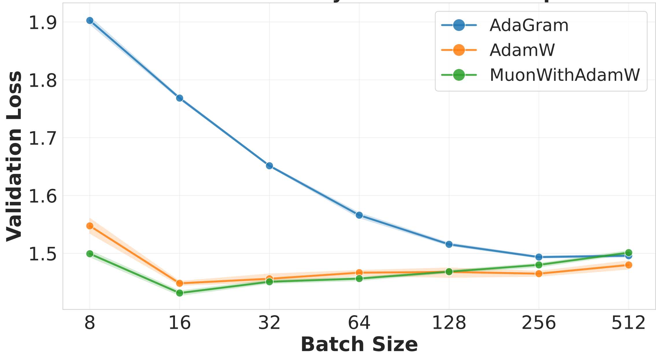
Best Validation Loss by Batch Size and Optimizer
