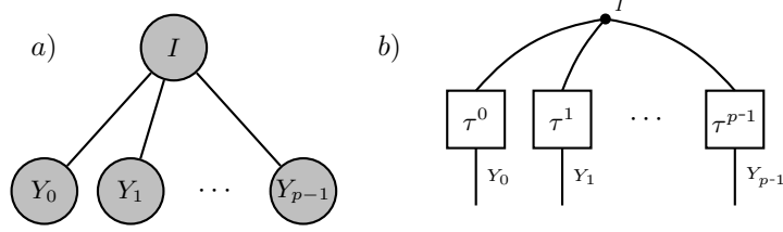
Figure 2: The CP tensor format consist in the CP hypergraph a) and decorating tensor networks b). Tensors in this format constructed as in Lem. 4 represent arbitrary faces.
