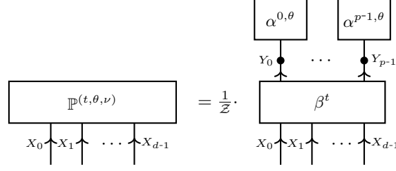
Figure 3: Representation of a member in an exponential family by a Computation-Activation Network with elementary activation. Here \mathcal{Z} \in \mathbb{R} is a normalization constant.
