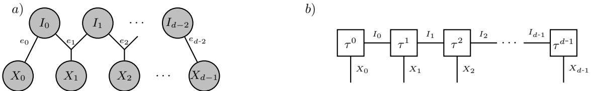
Figure 7: TT format consisting in the TT hypergraph a) and decorating tensor networks b).
