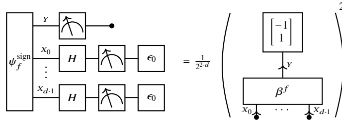
Fig. 11.12 Measurement setup for the Deutsch-Jozsa algorithm on the formula f .
