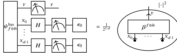
Fig. 11.13 Measurement setup for the inversion test on the formulas f and h . We measure the probability of the statistic qubit Y , when the distributed qubits X_{[d]} are in the ground state after a Walsh-Hadamard transform. This is equal to a scaled and squared contraction of the basis encoding to the formula f \oplus h .
