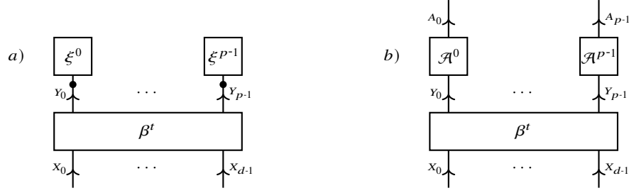
Fig. 17.1 Ancilla augmentation of an elementary Computation-Activation Network a) by replacing each leg vector of the elementary activation tensor by an directed ancilla augmentation.
