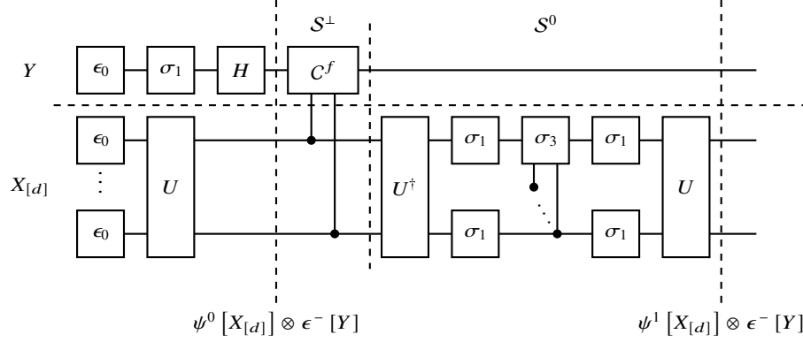
Fig. 11.17 Amplification scheme of the at the models of a Boolean function f supported coordinates of a quantum state. The ancilla variable Y is prepared as an disentangled Hadamard basis vector and stays disentangled during the following reflections. The oracle C^f effectively performs the reflection \mathcal{S}^\perp across the bad state supported at the models of f .
