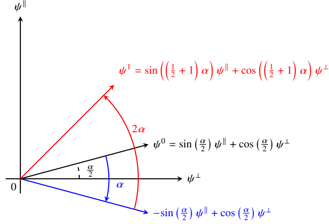
Fig. 11.14 Grover operator as a rotation in span (\psi^{\parallel}, \psi^{\perp}) .
