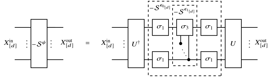
Fig. 11.15 Preparation of the negated reflection operator -S^{\psi} about a state \psi , which is prepared by a unitary U acting on the ground state \epsilon_{0[d]} [X_{[d]}] . The multiply controlled Pauli-Z is the negated reflection -S^{1[d]} , and extended to the negated reflection -S^{1[d]} about the ground state by adding layers of single qubit Pauli-X. When concatenating with U^{\dagger} and U , the -S^{\psi} results.
