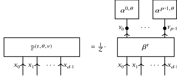
Fig. 13.3 Representation of a member of an exponential family by a Computation-Activation Network with elementary activation. Here Z \in \mathbb{R} is a normalization constant.
