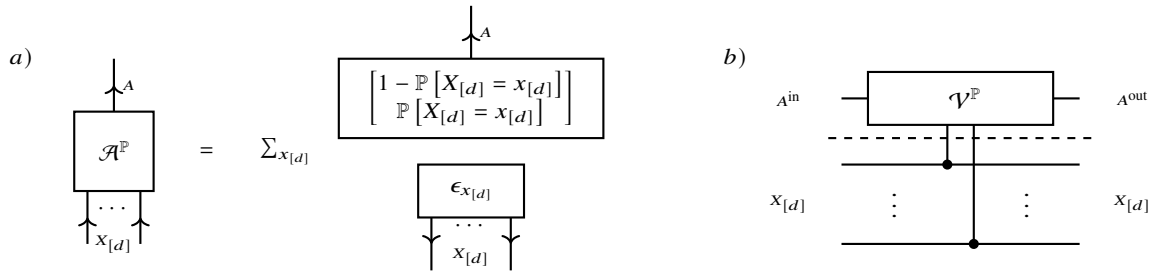
Fig. 1.4 Ancilla augmentation of a distribution \mathbb{P}[X_{[d]}] . a) Augmented distribution \mathcal{A}^{\mathbb{P}}[A, X_{[d]}] with the property that \mathbb{P}[X_{[d]}] = \mathcal{A}^{\mathbb{P}}[X_{[d]}|A = 1] . b) Preparation of the augmented distribution by the activation circuit of \mathbb{P}[X_{[d]}] .
