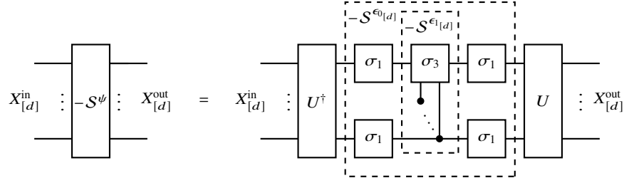
Fig. 12.15 Preparation of the negated reflection operator -\mathcal{S}^\psi about a state \psi , which is prepared by a unitary U acting on the ground state \epsilon_{0[d]} [X_{[d]}] . The multiply controlled Pauli-Z is the negated reflection -\mathcal{S}^{1[d]} , and extended to the negated reflection -\mathcal{S}^{1[d]} about the ground state by adding layers of single qubit Pauli-X. When concatenating with U^\dagger and U , the -\mathcal{S}^\psi results.
