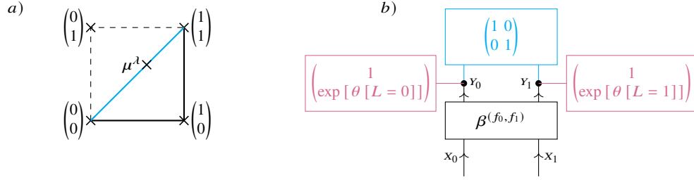
Fig. 14.5 a) Mean polytope of the statistic t = (X_0 \wedge X_1, X_0 \Rightarrow X_1) (thick), as a subset of the cube [0, 1]^2 (dashed). The blue line is the face of the polytope, which is not cube-like, that is not an intersection of the polytope with the faces of the hypercube. We further define for \lambda \in (0, 1) a mean parameter \mu_\lambda[L] = [\lambda \lambda]^T which is on the interior of the blue face. b) Corresponding Computation-Activation Network being the maximum entropy distribution reproducing \mu_\lambda[L] , when \lambda is the sigmoid of \theta[L = 0] + \theta[L = 1] .
