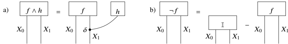
Fig. 9.4 Decomposition schemes by hybrid calculus, using coordinatewise transforms of tensors (see Def. ??). a) Conjunction performed by coordinatewise multiplications. b) Negations performed by coordinatewise subtraction from one.
