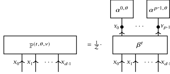
Fig. 14.3 Representation of a member of an exponential family by a Computation-Activation Network with elementary activation. Here Z \in \mathbb{R} is a normalization constant.
