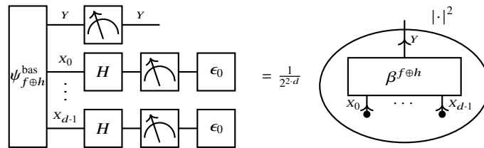
Fig. 12.13 Measurement setup for the inversion test on the formulas f and h . We measure the probability of the statistic qubit Y , when the distributed qubits X_{[d]} are in the ground state after a Walsh-Hadamard transform. This is equal to a scaled and squared contraction of the basis encoding to the formula f \oplus h .
