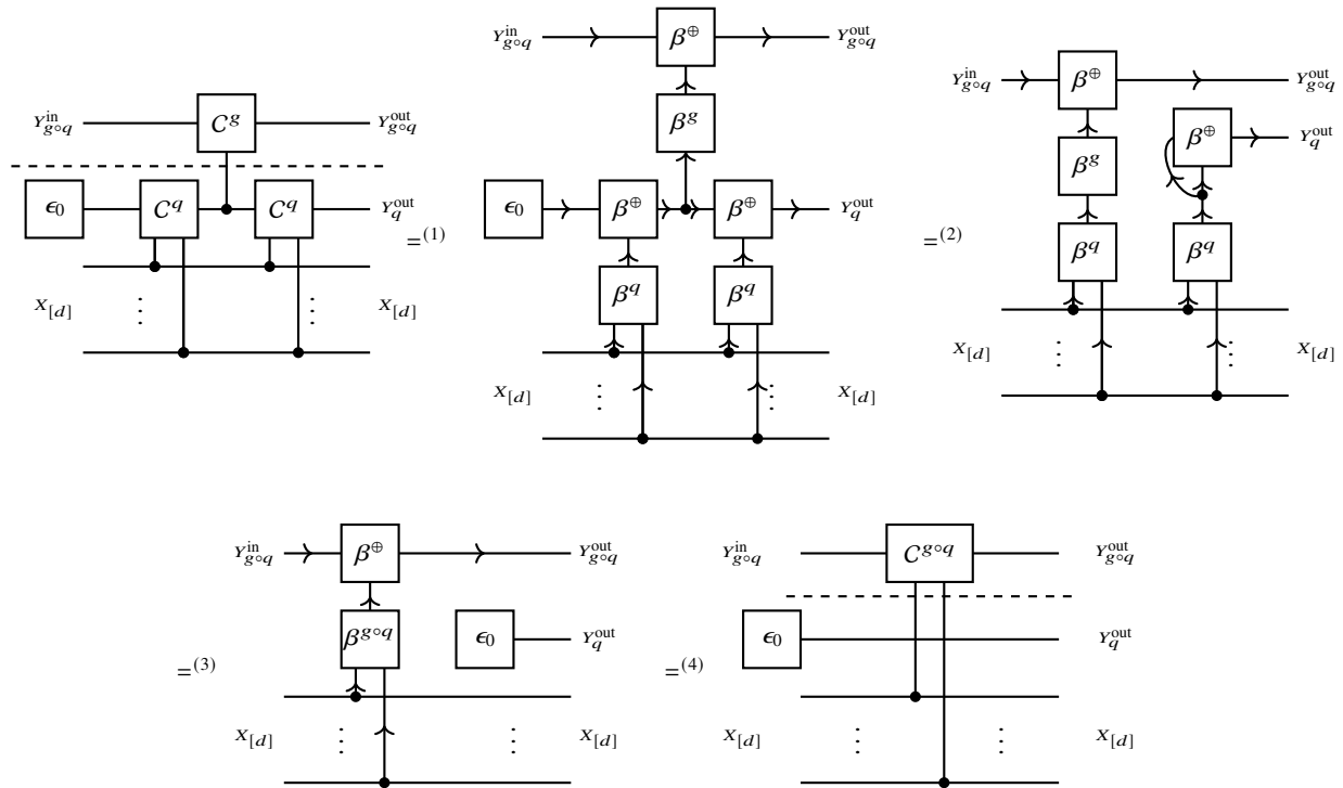
Fig. 12.8 Proof of Lem. 12.8 based on basis calculus.
