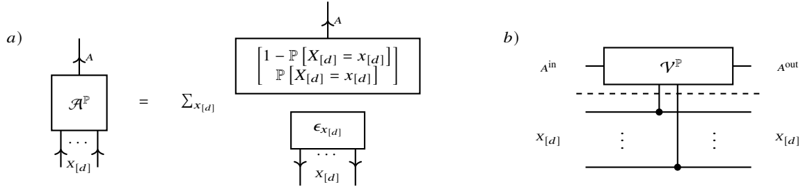
Fig. 12.4 Ancilla augmentation of a distribution \mathbb{P} [X_{[d]}] . a) Augmented distribution \mathcal{A}^{\mathbb{P}} [A, X_{[d]}] with the property that \mathbb{P} [X_{[d]}] = \mathcal{A}^{\mathbb{P}} [X_{[d]} | A = 1] . b) Preparation of the augmented distribution by the activation circuit of \mathbb{P} [X_{[d]}] .
