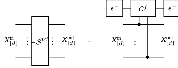
Fig. 12.16 Realization of the reflection across the subspace of one-hot encoded models to a Boolean function f . An ancilla qubit is prepared in the Hadamard basis state \epsilon^- and serves as the head qubit of the oracle C^f . By the phase kickback effect, the qubit stays disentangled and the reflection -S^{V^f} is effectively performed on the qubits X_{[d]} .
