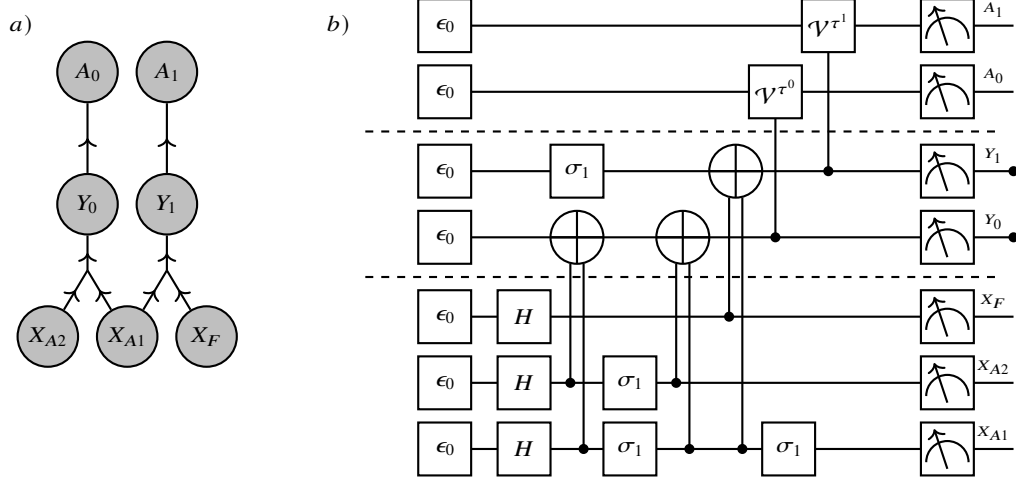
Fig. 18.4 Circuit to sample from the Computation-Activation Network in the toy accounting Example 18.1.
