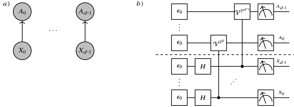
Fig. 12.5 Ancilla augmentation of an elementary distribution (which variables are pairwise independent). a) Hypergraph to the Bayesian Network representing the ancilla augmentation. b) Circuit preparing the ancilla augmented distribution by activation circuits acting on the disentangled initial state.
