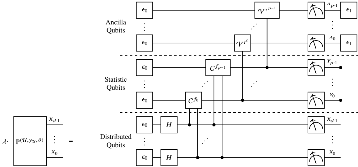
Fig. 18.3 Quantum Circuit to reproduce a q-sample of an augmented Computation-Activation Network. We measure the distributed qubits X_{[d]} and the ancilla qubits A_{[p]} and reject all samples, where an ancilla qubit is measured as 0.
