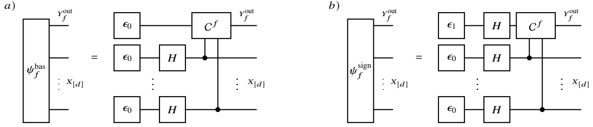
Fig. 12.11 Construction of the basis encoding state (a) and the sign encoding state (b) using the computation circuit of a function.
