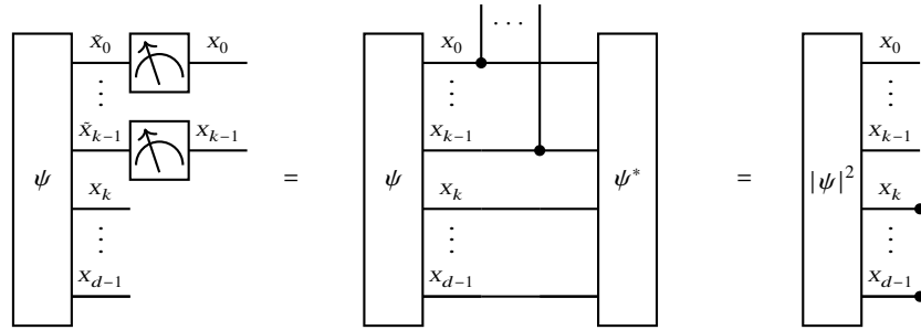
Fig. 12.1 Computational Basis Measurement of a quantum state \psi . The measurement symbols on the left side indicate the measured qubits and the first equation is understood as a definition. In the second equation we sketch, that the measurement distribution is equal to the contraction of the square absolute transform of \psi to the measured variables.
