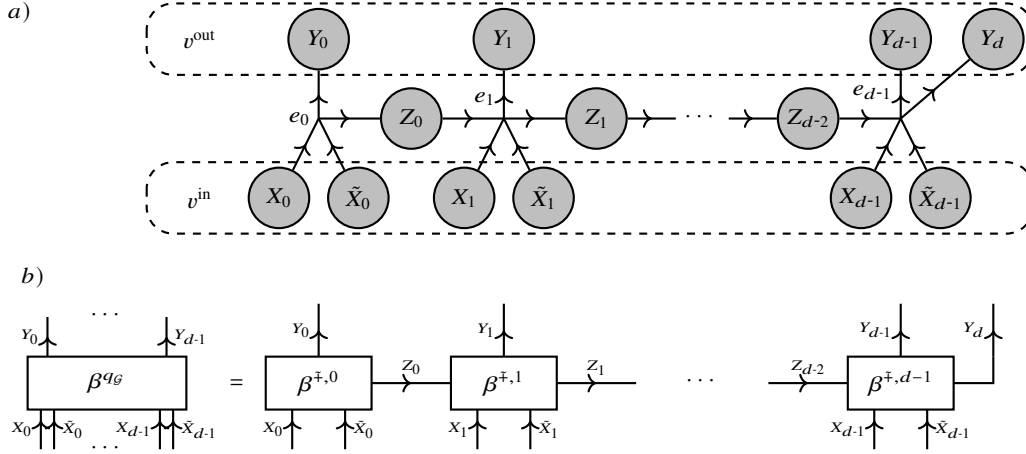
Fig. 9.2 Example of a decomposition hypergraph to the sum of integers (see Example 9.2). a) Hypergraph of directed edges e_k for k \in [d] , each decorated by an integer summation + preparing an index Y_k of the resulting sum. b) Corresponding tensor network decomposition of the basis encoded composition function, which is the sum of integers in m -adic representation.
