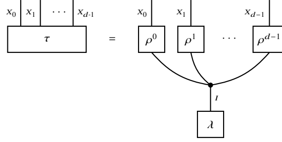
Fig. 10.1 Tensor Network diagram of a generic CP decomposition (see Def. 10.1)
