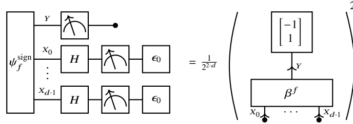
Fig. 12.12 Measurement setup for the Deutsch-Jozsa algorithm on the formula f .
