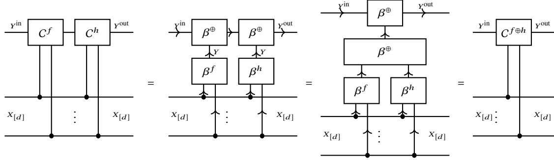
Fig. 12.9 Equivalence of the composition of computation circuits with the computation circuit of their mod2 sum (Lem. 12.9).
