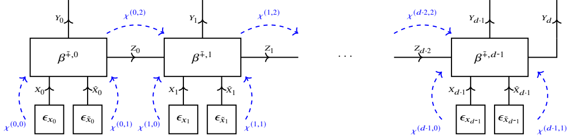
Fig. 9.3 Computation of the integer sum in m -adic representation by the Directed Belief Propagation Algorithm 7 (see Example 9.3). The summands are represented by one-hot encodings of the digits x_{[d]} and \tilde{x}_{[d]} , from which the messages start. The k -th digit (for k \in \{0, \dots, d-1\} ) of the sum is computed based on the first messages of the epoch labeled by \chi^{(k,[2])} . The third message \chi^{(k,2)} in each epoch communicates the carry bit to the next digit summation core. In the last message epoch the digit d-1 and d are computed based.
