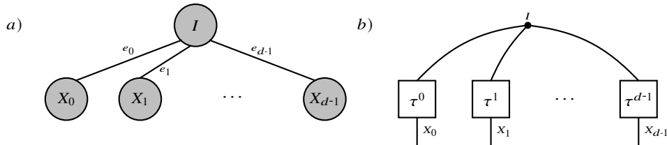
Fig. 1.1 Hypergraph to a CP format (see Example 1.2). a) Node-centric design. b) Corresponding tensor network on the edges of the hypergraph.
