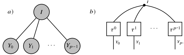
Fig. 14.2 The CP tensor format consist of the CP hypergraph a) and decorating tensor networks b). Tensors in this format constructed as in Lem. 14.4 represent arbitrary faces.
