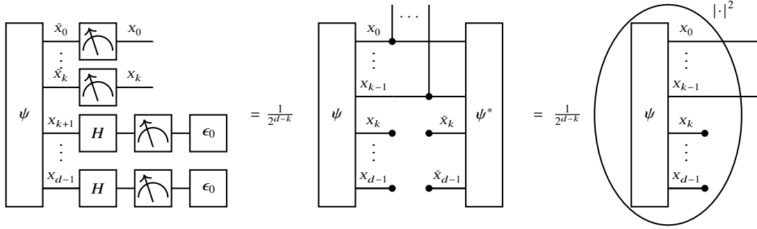
Fig. 12.2 Computational Basis Measurement of a quantum state \psi , after the Walsh-Hadamard Transform on the closed qubits. By the ellipse we indicate a coordinatewise transform to the square of the absolute, after the contraction.
