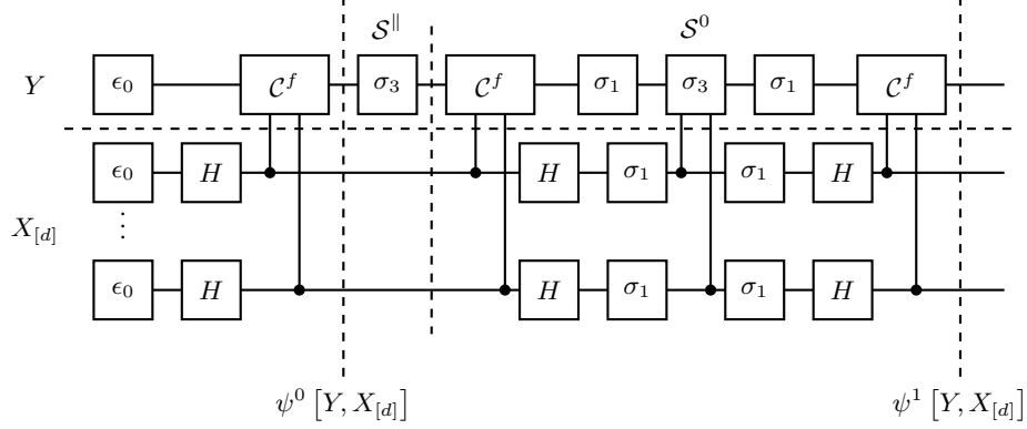
Figure 10: Amplitude amplifying circuit for the ancilla augmentation of a function f , for j = 1 repetitions. The initial state \psi^0 [Y, X_{[d]}] is the q-sample of the by Y augmented uniform distributions among the models of f , and prepared by action of the oracle C^f on the ground state. The amplification is then done by the Grover operator, which consists in the reflection S^{\parallel} across the state \psi^0 [Y, X_{[d]}] followed by a reflection reflection S^0 across the state \psi^0 [Y, X_{[d]}] .
