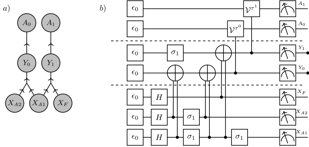
Figure 8: Circuit to sample from the Computation-Activation Network in the toy accounting Example 5. Note that a first Pauli-X gate \sigma_1 acting on X_{A2} can be omitted, since the prepared state is the Hadamard basis vector \epsilon^+ [X_{A2}] .
