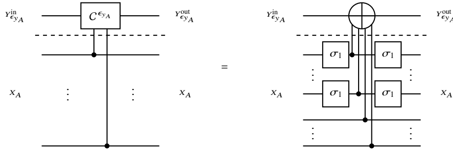
Fig. 11.9 Representation of a slice as a controlled CNOT gate. When the control state to a variable is 0, we introduce auxiliary Pauli-X gates.
