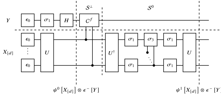
Fig. 11.15 Amplification scheme of the at the models of a Boolean function f supported coordinates of a quantum state. The ancilla variable Y is prepared as an disentangled Hadamard basis vector and stays disentangled during the following reflections. The oracle C^f effectively performs the reflection S^\perp across the bad state supported at the models of f .
