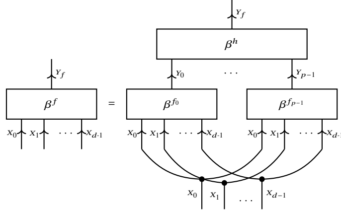
Fig. 10.1 Tensor network decomposition of the basis encoding of a function f , which is the composition of the functions f_0, \dots, f_{p-1} with a function h .
