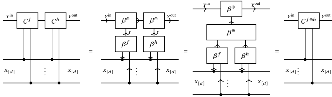
Fig. 11.8 Equivalence of the composition of computation circuits with the computation circuit of their mod2 sum (Lem. 11.8).
