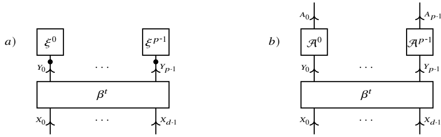
Fig. 17.1 Ancilla augmentation of an elementary Computation-Activation Network a) by replacing each leg vector of the elementary activation tensor by an directed ancilla augmentation.
