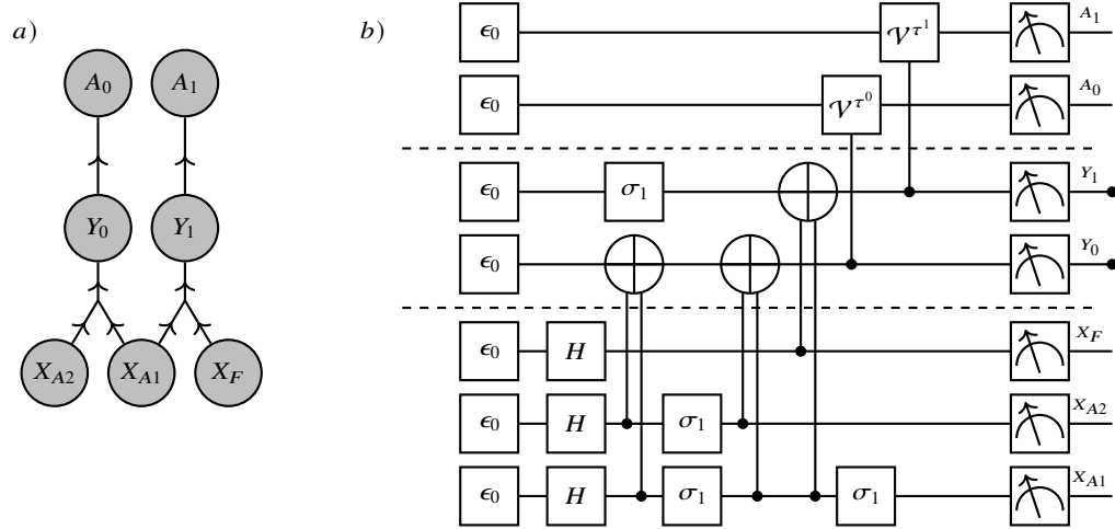
Fig. 17.4 Circuit to sample from the Computation-Activation Network in the toy accounting Example 17.1.
