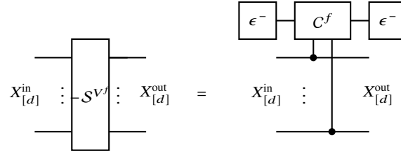
Fig. 11.14 Realization of the reflection across the subspace of one-hot encoded models to a Boolean function f . An ancilla qubit is prepared in the Hadamard basis state \epsilon^- and serves as the head qubit of the oracle C^f . By the phase kickback effect, the qubit stays disentangled and the reflection -S^{V^f} is effectively performed on the qubits X_{[d]} .
