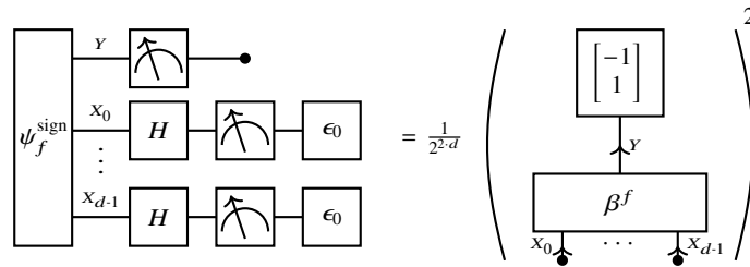
Fig. 11.16 Measurement setup for the Deutsch-Jozsa algorithm on the formula f .
