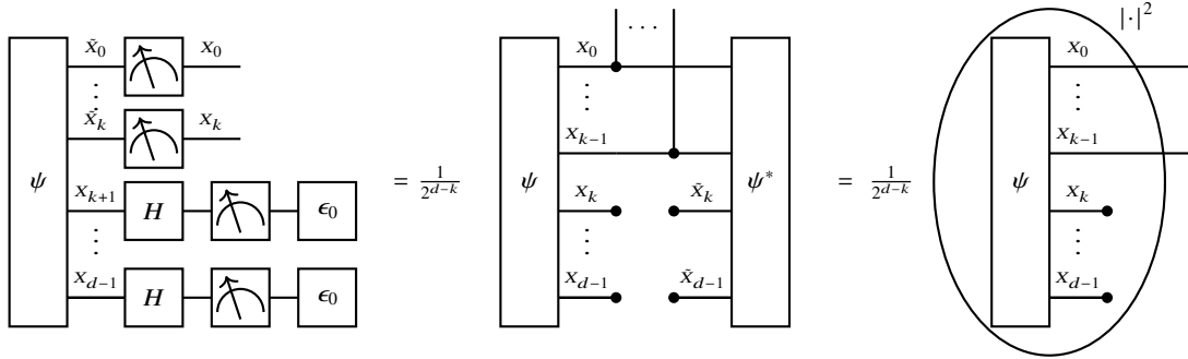
Fig. 11.2 Computational Basis Measurement of a quantum state \psi , after the Walsh-Hadamard Transform on the closed qubits. By the ellipse we indicate a coordinatewise transform to the square of the absolute, after the contraction.
