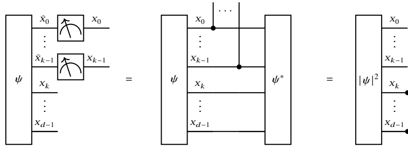
Fig. 11.1 Computational Basis Measurement of a quantum state \psi . The measurement symbols on the left side indicate the measured qubits and the first equation is understood as a definition. In the second equation we sketch, that the measurement distribution is equal to the contraction of the square absolute transform of \psi to the measured variables.
