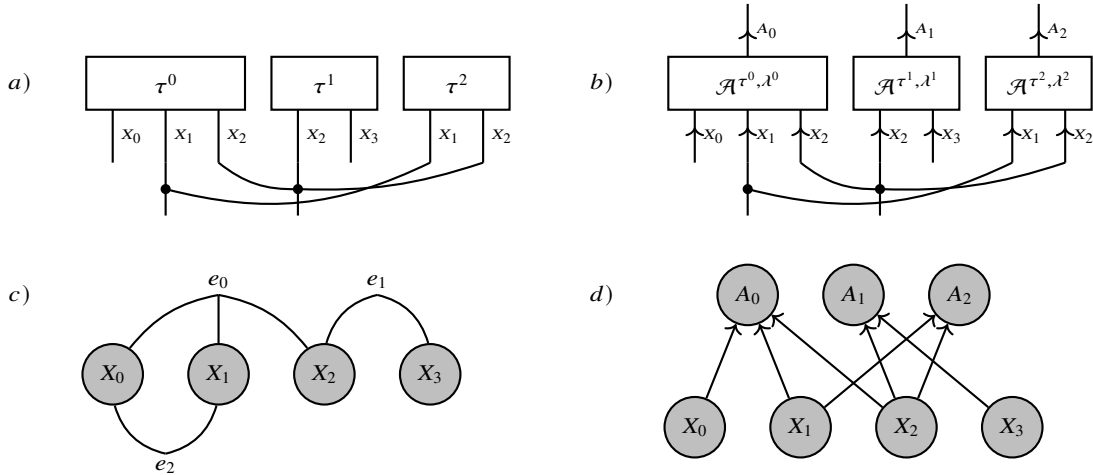
Fig. 11.6 Ancilla augmentation of a Markov Network a) onto a Bayesian Network b). To this end the arbitrary non-negative cores \tau^e are replaced by directed ancilla augmented cores \tilde{\tau}^e , with ancillary variables outgoing.
