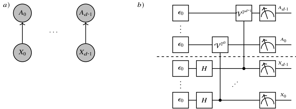
Fig. 11.5 Ancilla augmentation of an elementary distribution (which variables are pairwise independent). a) Hypergraph to the Bayesian Network representing the ancilla augmentation. b) Circuit preparing the ancilla augmented distribution by activation circuits acting on the disentangled initial state.
