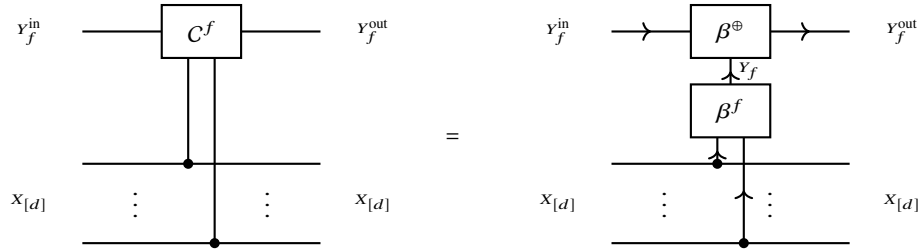
Fig. 11.7 Relation of computation circuit and basis encodings. The computation circuit of a function is the contraction of its basis encoding with the basis encoding of the mod2 sum \oplus .
