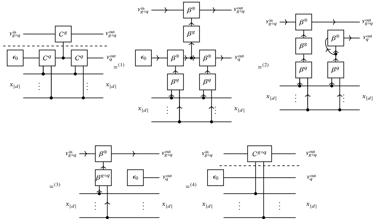
Fig. 11.10 Proof of Lem. 11.11 based on basis calculus.
