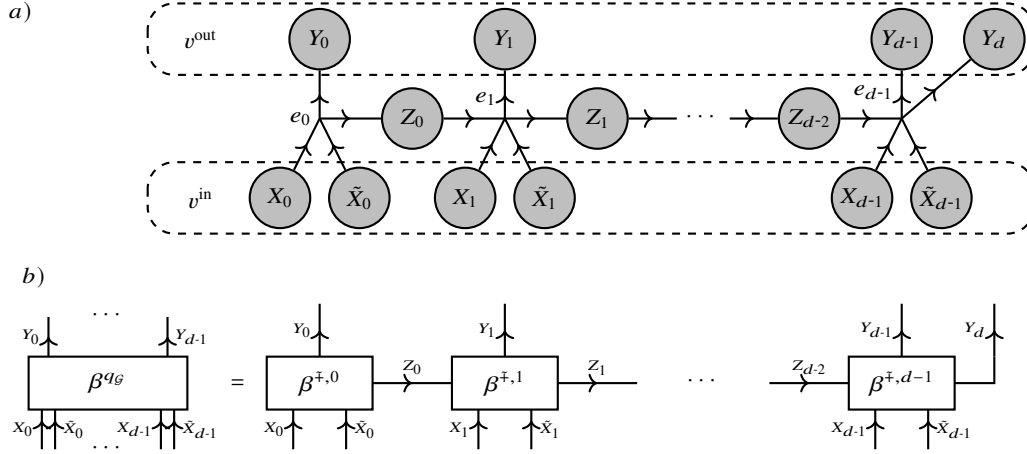
Fig. 10.2 Example of a decomposition hypergraph to the sum of integers (see Example 10.1). a) Hypergraph of directed edges e_k for k \in [d] , each decorated by an integer summation + preparing an index Y_k of the resulting sum. b) Corresponding tensor network decomposition of the basis encoded composition function, which is the sum of integers in m -adic representation.
