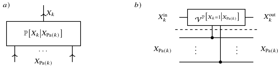
Fig. 11.3 Representation of directed and positive tensor by a controlled rotation. a) Conditional probability tensor \mathbb{P}[X_k | X_{\text{Pa}(k)}] being a tensor in a Bayesian Network. b) Circuit Encoding as a controlled rotation, which is the Activation circuit of the tensor \mathbb{P}[X_k = 1 | X_{\text{Pa}(k)}] .
