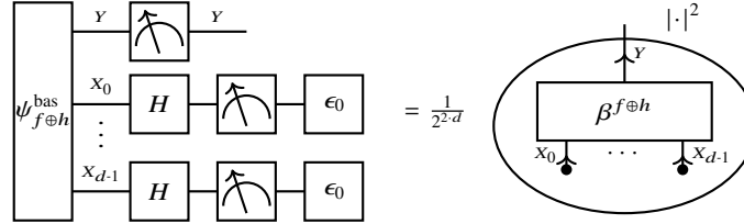
Fig. 11.17 Measurement setup for the inversion test on the formulas f and h . We measure the probability of the statistic qubit Y , when the distributed qubits X_{[d]} are in the ground state after a Walsh-Hadamard transform. This is equal to a scaled and squared contraction of the basis encoding to the formula f \oplus h .
