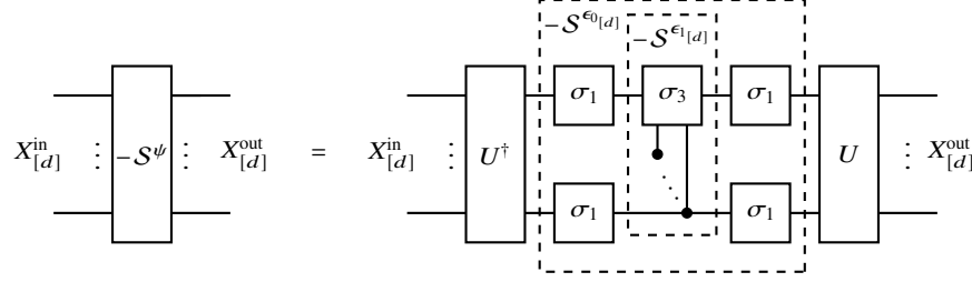
Fig. 1.13 Preparation of the negated reflection operator -\mathcal{S}^\psi about a state \psi , which is prepared by a unitary U acting on the ground state \epsilon_{0[d]} [X_{[d]}] . The multiply controlled Pauli-Z is the negated reflection -\mathcal{S}^{1[d]} , and extended to the negated reflection -\mathcal{S}^{\epsilon_{1[d]}} about the ground state by adding layers of single qubit Pauli-X. When concatenating with U^\dagger and U , the -\mathcal{S}^\psi results.
