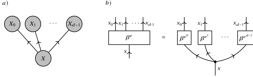
Fig. 3.1 Representation of a categorical constraint in a CP Format tensor network. a) Representation of the dependency of the graphical model. b) Tensor Representation with further network decomposition.
