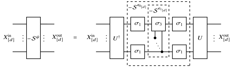
Fig. 1.13 Preparation of the negated reflection operator -S^\psi about a state \psi , which is prepared by a unitary U acting on the ground state \epsilon_{0[d]} [X_{[d]}] . The multiply controlled Pauli-Z is the negated reflection -S^{1[d]} , and extended to the negated reflection -S^{\epsilon_1[d]} about the ground state by adding layers of single qubit Pauli-X. When concatenating with U^\dagger and U , the -S^\psi results.
