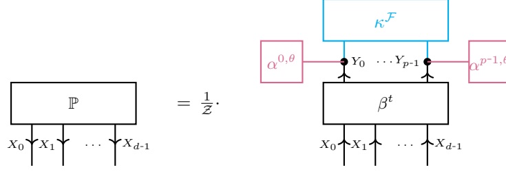
Figure 2: Tensor network decomposition of maximum entropy distributions to the constraint \mu[L] = \langle \mathbb{P}[X_{[d]}], \sigma^t[X_{[d]}, L] \rangle_{[L]} . Blue: Boolean tensor \kappa^{\mathcal{F}}[Y_{[p]}] dependent on the face \mathcal{F}(\cdot)\mu , which represents the refinement of the base measure to the face, and is possibly non-elementary. Red: Elementary activation tensor \alpha^\theta[Y_{[p]}] = \bigotimes_{s \in [n]} \alpha^{\ell, \theta}[Y_\ell] to the weight \theta[L] = B^{t, \nu^{t, \mathcal{F}}}(\mu) .
