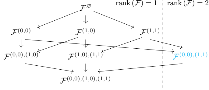
Figure 4: Face lattice L((X_0 \wedge X_1, X_0 \Rightarrow X_1)) to Example 7. The directed arrows represent inclusion of the faces, which is a partial order of the faces. The face \mathcal{F}^{(0,0),(1,1)} is the only face, which is not representable by an elementary hypergraph. It is representable in a CP with hidden rank 2
