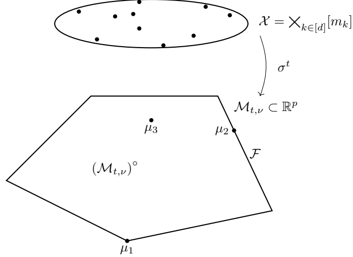
Figure 1: Sketch of the statistic mapping the states to the mean parameters.
