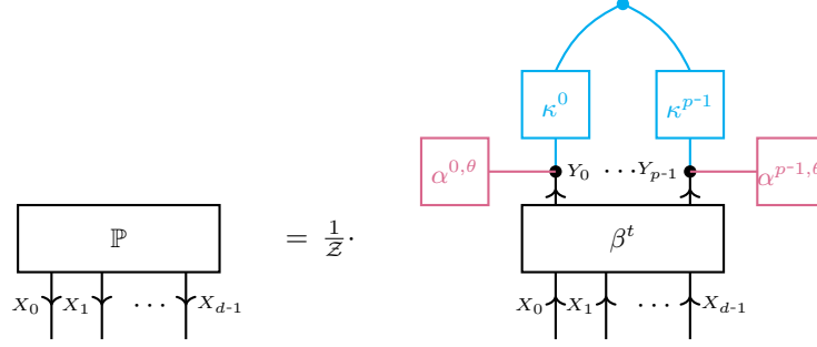
Figure 3: Tensor network decomposition of maximum entropy distributions to the constraint \mu[L] = \langle \mathbb{P}[X_{[d]}], \sigma^t[X_{[d]}, L] \rangle_{[L]} . Blue: Constraint activation cores \kappa^\ell in a CP decomposition, representing the face measure to the minimal face, such that \mu \in \mathcal{F}^\mathcal{F} . Red: Probabilistic activation cores \alpha^{\ell, \theta}[Y_\ell] in an elementary decomposition, where each leg core is a scaled exponentials evaluated on the enumerated image \text{im}(t_\ell) .
