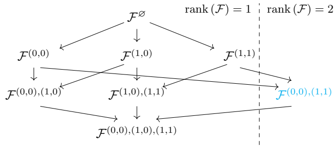
Figure 5: Face lattice L((X_0 \wedge X_1, X_0 \Rightarrow X_1)) to Example 5. The directed arrows represent inclusion of the faces, which is a partial order of the faces. The face \mathcal{F}^{(0,0),(1,1)} is the only face, which is not representable by an elementary hypergraph. It is representable in a CP with hidden rank 2
