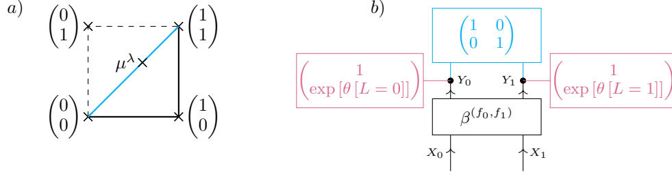
Figure 4: a) Mean polytope of the statistic \mathcal{F} = (X_0 \wedge X_1, X_0 \Rightarrow X_1) (thick), as a subset of the cube [0, 1]^2 (dashed). The blue line is the face of the polytope, which is not cube like, that is not an intersection of the polytope with the faces of the polytope. We further define for \lambda \in (0, 1) a mean parameter \mu_\lambda[L] = [\lambda \lambda]^T which is on the interior of the blue face. b) Corresponding Computation-Activation Network being the maximum entropy distribution reproducing \mu_\lambda[L] , when \lambda is the sigmoid of \theta[L = 0] + \theta[L = 1] .
