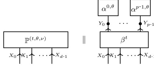
Figure 2: Representation of a member in an exponential family by a Computation-Activation Network with elementary activation. Since the right hand side is not normalized both sides are equal up to a constant.
