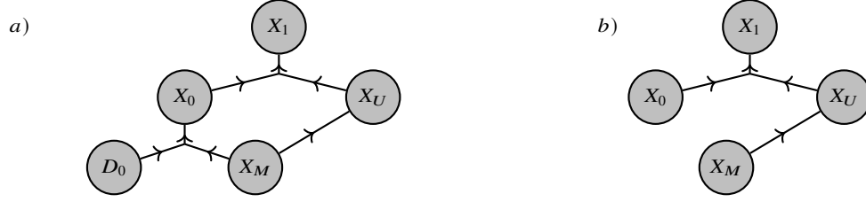
Fig. 6.5 Causal graph for the Backdoor Criterion (see Def. 6.2). a) The mediator variable X_M blocks any backdoor path from X_0 to X_1 , potentially through a confounding variable X_U . b) The effect of the intervention on X_0 reduces the Bayesian network effectively to the shown subgraph.
