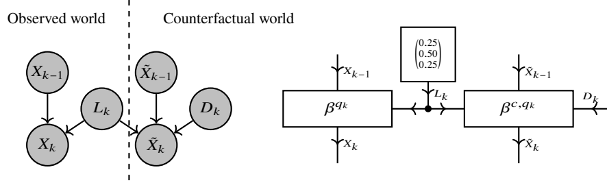
Fig. 1.9 Part of the counterfactual twinned network for the random walk (see Example 1.6 and Example 1.7).
