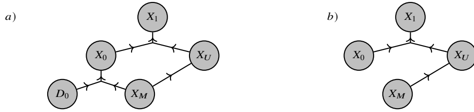
Fig. 1.5 Causal graph for the Backdoor Criterion (see Def. 1.2). a) The mediator variable X_M blocks any backdoor path from X_0 to X_1 , potentially through a confounding variable X_U . b) The effect of the intervention on X_0 reduces the Bayesian network effectively to the shown subgraph.
