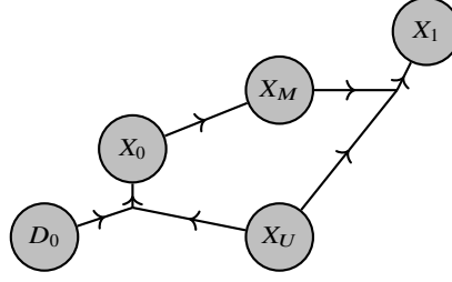
Fig. 1.6 Typical hypergraph, where X_M satisfies the frontdoor criterion with respect to X_0 and X_1 .
