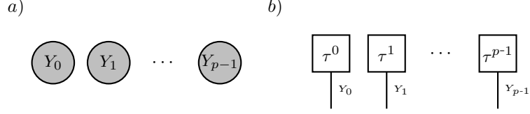
Fig. 1 Elementary tensor format consisting of the elementary hypergraph EL a ), and corresponding tensor networks b ) being the tensor products of vectors.
