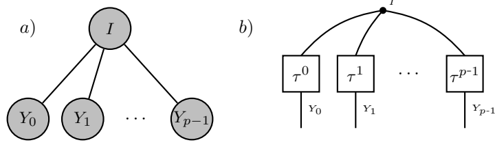
Fig. 2 The CP tensor format consist of the CP hypergraph a) and decorating tensor networks b). Tensors in this format constructed as in Lem. 4 represent arbitrary faces.
