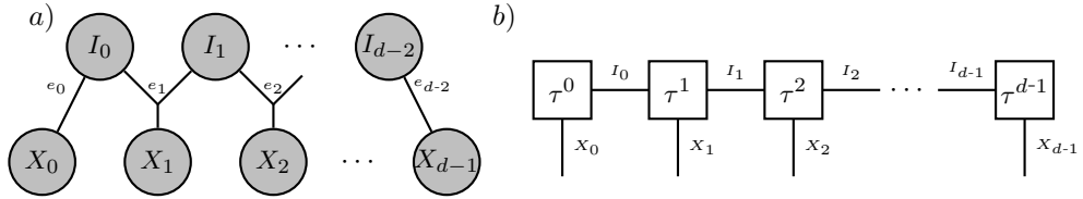
Fig. 7 TT format consisting of the TT hypergraph a) and decorating tensor networks b).
