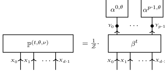
Fig. 3 Representation of a member of an exponential family by a Computation-Activation Network with elementary activation. Here \mathcal{Z} \in \mathbb{R} is a normalization constant.
