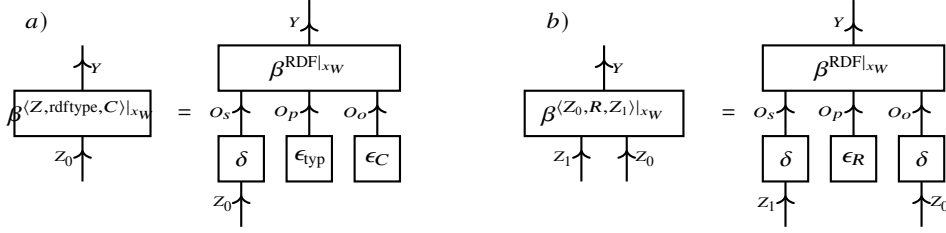
Fig. 4.3 Triple patterns of SPARQL as tensor networks. a) Example of unary triple pattern \langle Z, \text{rdf:type}, C \rangle specifying whether an individual I_{o_1} is a member of class C . b) Example of a binary triple pattern \langle Z_0, R, Z_1 \rangle specifying whether individuals I_{o_1} and I_{o_2} have a relation R . By \epsilon_{\text{type}}, \epsilon_C, \epsilon_R we denote the one-hot encodings of the enumeration of the resources \text{rdf:type}, C and R .
