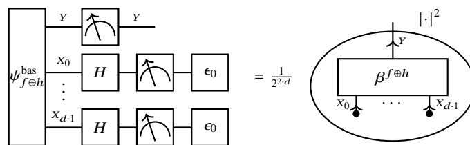
Fig. 12.13 Measurement setup for the inversion test on the formulas f and h . We measure the probability of the statistic qubit Y , when the distributed qubits X_{[d]} are in the ground state after a Walsh-Hadamard transform. This is equal to a scaled and squared contraction of the basis encoding to the formula f \oplus h .
