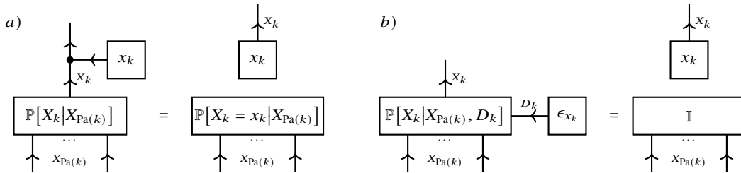
Fig. 6.5 Comparison of conditioning (a) and intervention (b) on a variable X_k . When intervening, a trivial tensor over the parent variables is left, which can be exploited for further query simplifications.
