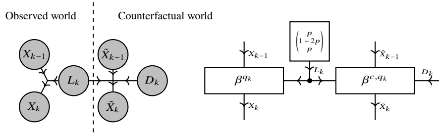
Fig. 6.10 Part of the counterfactual twinned network for the random walk (see Example ?? and Example ??).
