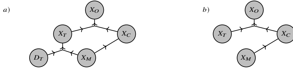
Fig. 6.6 Causal graph for the Backdoor Criterion (see Def. 6.2). a) The mediator variable X_M blocks any backdoor path from X_T to X_O , potentially through a confounding variable X_C . b) The effect of the intervention on X_T reduces the Bayesian network effectively to the shown subgraph.
