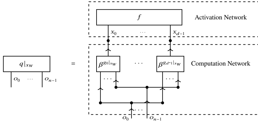
Fig. 4.1 Grounding of a quantifier-free first-order logic formula q is a Computation-Activation Network: The atomic formulas g_k are computed and activated by a propositional formula f [X_{[d]}] . The computation network therefore consists of the (possibly substituted) predicate groundings, while the activation network consists of the (possibly decomposed) propositional formula f [X_{[d]}] .
