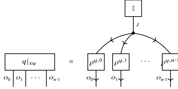
Fig. 4.3 Basis CP Decomposition of the grounding of q , following the scheme of Thm. 10.1. Instead of direct storage of the grounding tensor q|_{x_W} , the non-zero coordinates are enumerated by a variable J and the corresponding coordinates stored in leg-matrices \rho^{q,l} .
