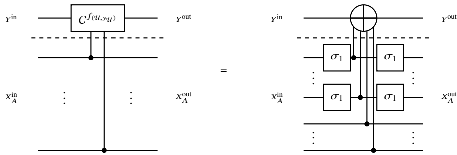
Fig. 12.10 Computation circuit to a MPRM term f_{(\mathcal{U}, y_{\mathcal{U}})} , consisting in a multiple controlled NOT gate and Pauli-X gates for legs with y_k = 0 .
