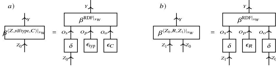
Fig. 4.2 Triple patterns of SPARQL as tensor networks. a) Example of unary triple pattern \langle Z, \text{rdf:type}, C \rangle specifying whether an individual I_{o_1} is a member of class C . b) Example of a binary triple pattern \langle Z_0, R, Z_1 \rangle specifying whether individuals I_{o_1} and I_{o_2} have a relation R . By \epsilon_{\text{typ}} , \epsilon_C , \epsilon_R we denote the one-hot encodings of the enumeration of the resources \text{rdf:type} , C and R .
