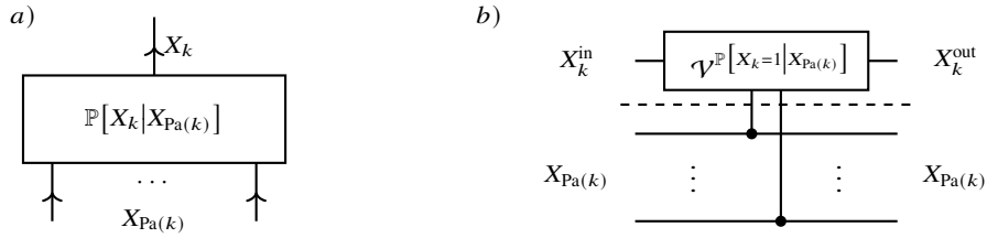
Fig. 12.3 Representation of directed and positive tensor by a controlled rotation. a) Conditional probability tensor \mathbb{P}[X_k | X_{\text{Pa}(k)}] being a tensor in a Bayesian Network. b) Circuit Encoding as a controlled rotation, which is the Activation circuit of the tensor \mathbb{P}[X_k = 1 | X_{\text{Pa}(k)}] .
