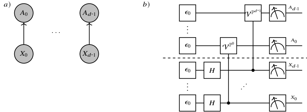
Fig. 13.5 Ancilla augmentation of an elementary distribution (which variables are pairwise independent). a) Hypergraph to the Bayesian Network representing the ancilla augmentation. b) Circuit preparing the ancilla augmented distribution by activation circuits acting on the disentangled initial state.
