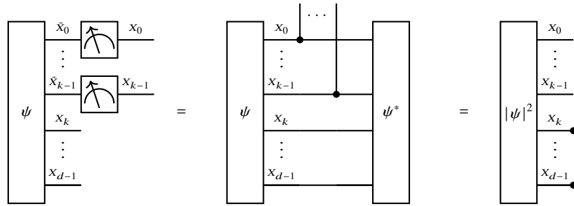
Fig. 13.1 Computational Basis Measurement of a quantum state \psi . The measurement symbols on the left side indicate the measured qubits and the first equation is understood as a definition. In the second equation we sketch, that the measurement distribution is equal to the contraction of the square absolute transform of \psi to the measured variables.
