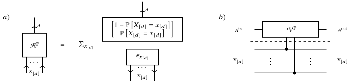
Fig. 13.4 Ancilla augmentation of a distribution \mathbb{P} [X_{[d]}] . a) Augmented distribution \mathcal{A}^{\mathbb{P}} [A, X_{[d]}] with the property that \mathbb{P} [X_{[d]}] = \mathcal{A}^{\mathbb{P}} [X_{[d]} | A = 1] . b) Preparation of the augmented distribution by the activation circuit of \mathbb{P} [X_{[d]}] .
