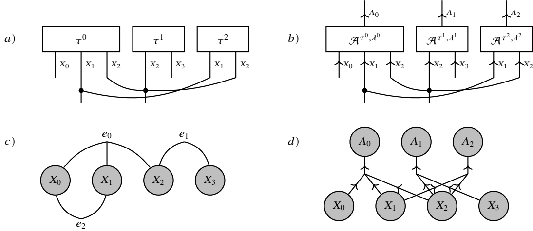
Fig. 13.6 Ancilla augmentation of a Markov Network a) onto a Bayesian Network b). To this end the arbitrary non-negative cores \tau^e are replaced by directed ancilla augmented cores \tilde{\tau}^e , with ancilly variables outgoing.
