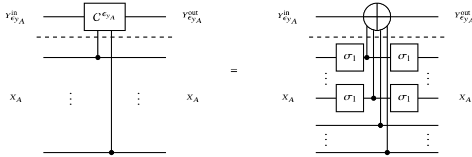
Fig. 13.9 Representation of a slice as a controlled CNOT gate. When the control state to a variable is 0, we introduce auxiliary Pauli-X gates.
