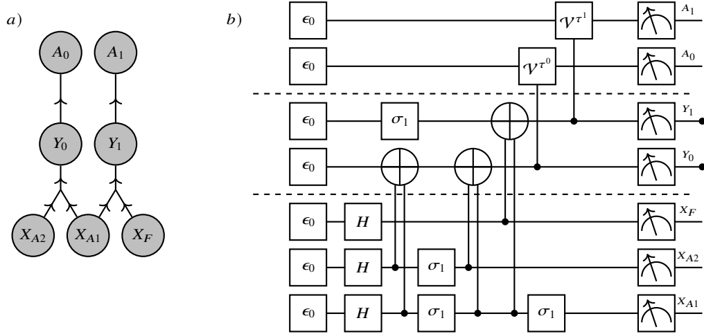
Fig. 19.4 Circuit to sample from the Computation-Activation Network in the toy accounting Example 19.1.
