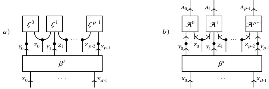
Fig. 19.2 Ancilla augmentation of an TT Computation-Activation Network a) by a Bayesian Network b). The hidden variables in the TT activation tensor are treated as distributed variables. Marginalization over the hidden variables and conditioning on the activation variables in state 1, we reproduce the Computation-Activation Network.
