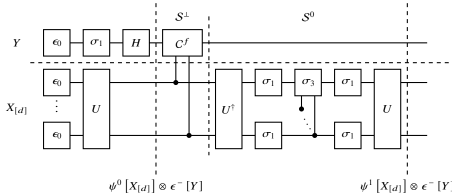
Fig. 13.17 Amplification scheme of the at the models of a Boolean function f supported coordinates of a quantum state. The ancilla variable Y is prepared as an disentangled Hadamard basis vector and stays disentangled during the following reflections. The oracle C^f effectively performs the reflection S^\perp across the bad state supported at the models of f .
