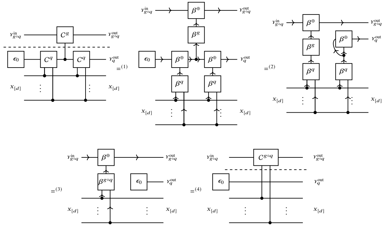
Fig. 13.10 Proof of Lem. 13.11 based on basis calculus.
