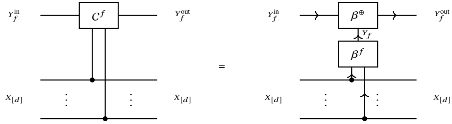
Fig. 13.7 Relation of computation circuit and basis encodings. The computation circuit of a function is the contraction of its basis encoding with the basis encoding of the mod2 sum \oplus .
