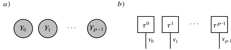
Fig. 15.1 Elementary tensor format consisting of the elementary hypergraph EL a) , and corresponding tensor networks b) being the tensor products of vectors.
