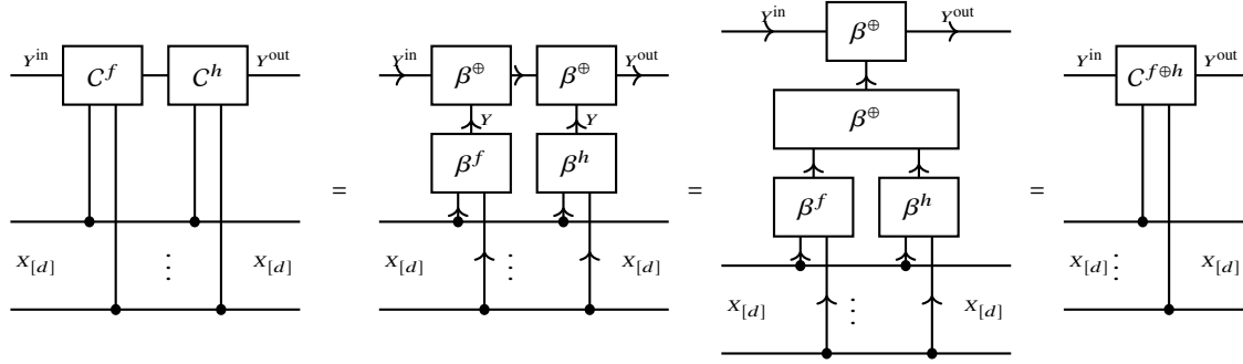
Fig. 13.8 Equivalence of the composition of computation circuits with the computation circuit of their mod2 sum (Lem. 13.8).
