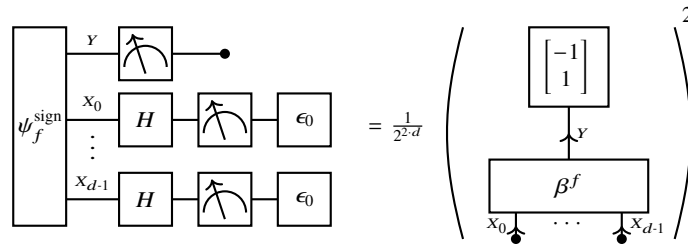
Fig. 13.12 Measurement setup for the Deutsch-Jozsa algorithm on the formula f .
