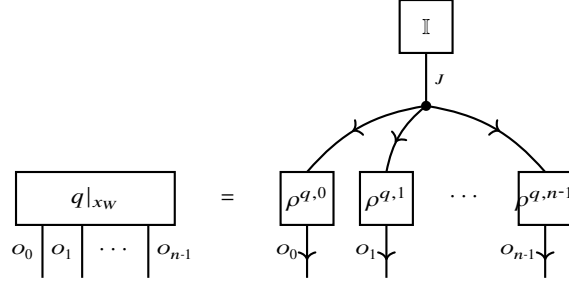
Fig. 4.1 Basis CP Decomposition of the grounding of q , following the scheme of Thm. 11.1. Instead of direct storage of the grounding tensor q|_{x_W} , the non-zero coordinates are enumerated by a variable J and the corresponding coordinates stored in leg-matrices \rho^{q,l} .
