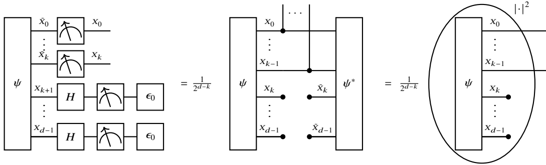
Fig. 13.2 Computational Basis Measurement of a quantum state \psi , after the Walsh-Hadamard Transform on the closed qubits. By the ellipse we indicate a coordinatewise transform to the square of the absolute, after the contraction.
