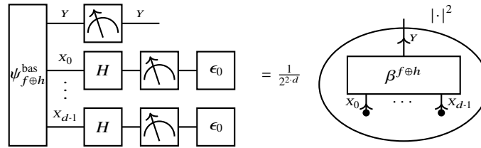
Fig. 13.13 Measurement setup for the inversion test on the formulas f and h . We measure the probability of the statistic qubit Y , when the distributed qubits X_{[d]} are in the ground state after a Walsh-Hadamard transform. This is equal to a scaled and squared contraction of the basis encoding to the formula f \oplus h .
