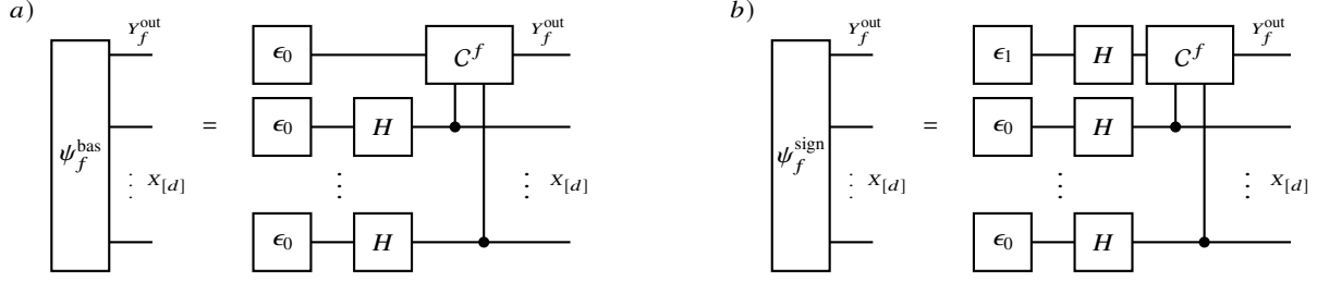
Fig. 13.11 Construction of the basis encoding state (a) and the sign encoding state (b) using the computation circuit of a function.
