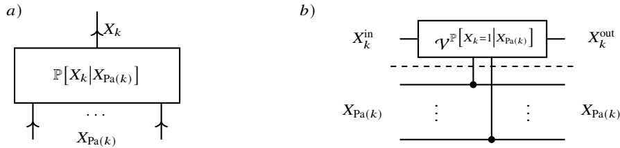
Fig. 13.3 Representation of directed and positive tensor by a controlled rotation. a) Conditional probability tensor \mathbb{P}[X_k | X_{\text{Pa}(k)}] being a tensor in a Bayesian Network. b) Circuit Encoding as a controlled rotation, which is the Activation circuit of the tensor \mathbb{P}[X_k = 1 | X_{\text{Pa}(k)}] .
