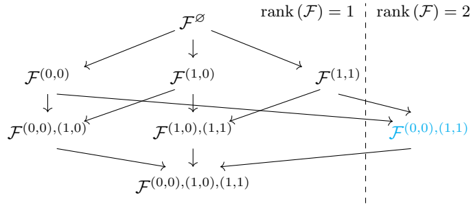
Figure 5: Face lattice L((X_0 \wedge X_1, X_0 \Rightarrow X_1)) to Example 7. The directed arrows represent inclusion of the faces, which is a partial order of the faces. The face \mathcal{F}^{(0,0),(1,1)} is the only face, which is not representable by an elementary hypergraph. It is representable in a CP with hidden rank 2
