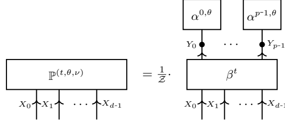
Figure 2: Representation of a member in an exponential family by a Computation-Activation Network with elementary activation. Here Z \in \mathbb{R} is a normalization constant.
