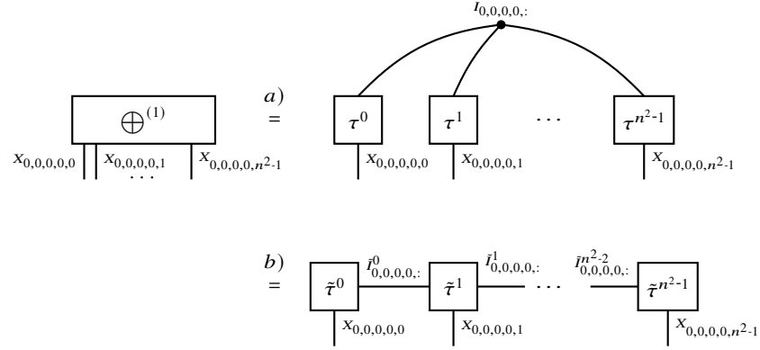
Fig. 3.2 Decomposition of the position constraint \bigoplus^{(1)} at position (r_0, r_1, c_0, c_1) = (0, 0, 0, 0) into a) a CP decomposition with hidden variable I_{0,0,0,0,:} and b) a TT decomposition with d - 1 hidden variables I_{0,0,0,0,:}^k, k \in [d - 1] .
