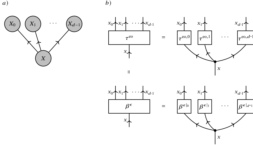
Fig. 3.1 Representation of an exactly-one constraint in a CP Format tensor network.
