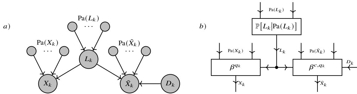
Fig. 6.4 Counterfactual twinned network: a) as a Bayesian network. b) Decorations by causal augmented basis encodings by a do-variable for X_k , a conditional probability distribution for L_k and a basis encoding for the counterfactual variable \tilde{X}_k .
