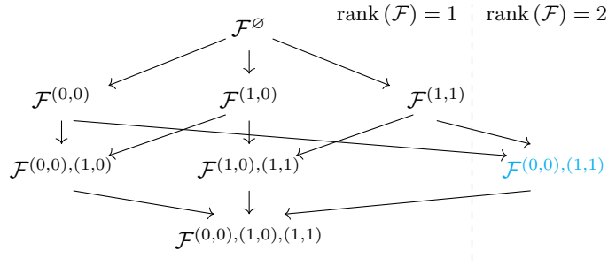
Figure 6: Face lattice L((X_0 \wedge X_1, X_0 \Rightarrow X_1)) to Example 7. The directed arrows represent inclusion of the faces, which is a partial order of the faces. The face \mathcal{F}^{(0,0),(1,1)} is the only face, which is not representable by an elementary hypergraph. It is representable in a CP with hidden rank 2
