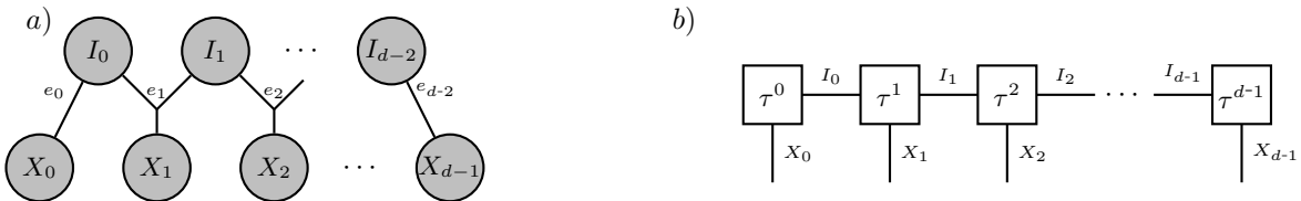
Figure 7: TT format consisting of the TT hypergraph a) and decorating tensor networks b).
