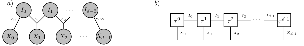
Fig. 7 TT format consisting of the TT hypergraph a) and decorating tensor networks b).
