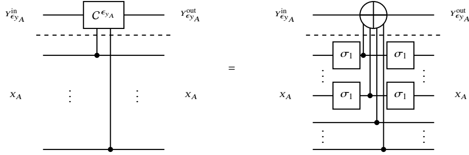
Fig. 8.9 Representation of an slice as a controlled CNOT gate. When the control state to a variable is 0, we introduce auxiliary Pauli-X gates.
