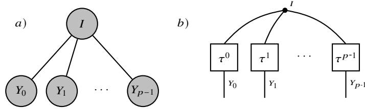
Fig. 10.2 The CP tensor format consist of the CP hypergraph a) and decorating tensor networks b). Tensors in this format constructed as in Lem. 10.4 represent arbitrary faces.
