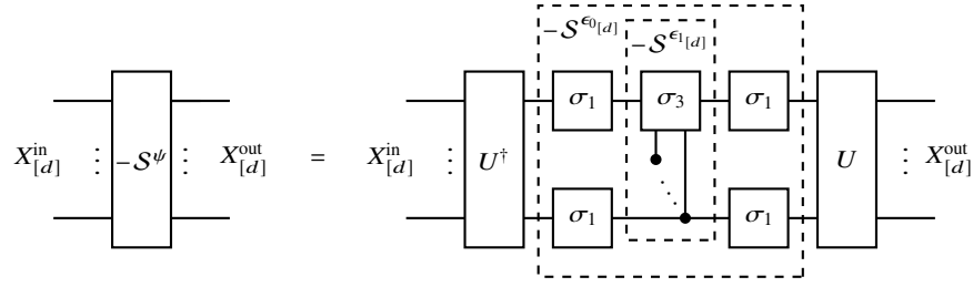
Fig. 1.13 Preparation of the negated reflection operator -\mathcal{S}^\psi about a state \psi , which is prepared by a unitary U acting on the ground state \epsilon_{0[d]} [X_{[d]}] . The multiply controlled Pauli-Z is the negated reflection -\mathcal{S}^{1[d]} , and extended to the negated reflection -\mathcal{S}^{1[d]} about the ground state by adding layers of single qubit Pauli-X. When concatenating with U^\dagger and U , the -\mathcal{S}^\psi results.
