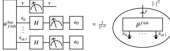
Fig. 1.17 Measurement setup for the inversion test on the formulas f and h . We measure the probability of the statistic qubit Y , when the distributed qubits X_{[d]} are in the ground state after a Walsh-Hadamard transform. This is equal to a scaled and squared contraction of the basis encoding to the formula f \oplus h .
