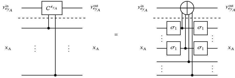
Fig. 1.9 Representation of an slice as a controlled CNOT gate. When the control state to a variable is 0, we introduce auxiliary Pauli-X gates.
