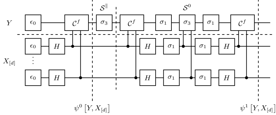
Figure 10: Amplitude amplifying circuit for the ancilla augmentation of a function f , for j = 1 repetitions. The initial state \psi^0 [Y, X_{[d]}] is the q -sample of the by Y augmented uniform distributions among the models of f , and prepared by action of the oracle C^f on the ground state. The amplification is then done by the Grover operator, which consists in the reflection S^{\parallel} across the state \psi^{\parallel} [Y, X_{[d]}] followed by a reflection reflection S^0 across the state \psi^0 [Y, X_{[d]}] .
