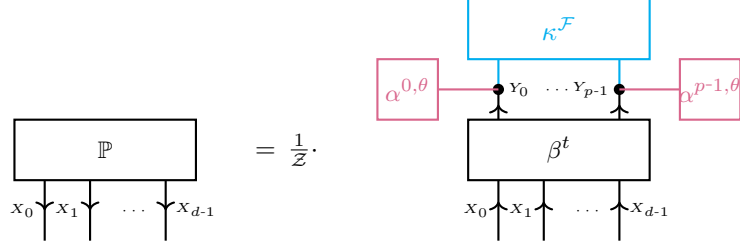
Fig. 4 Tensor network decomposition of maximum entropy distributions to the constraint \mu[L] = \langle \mathbb{P}[X_{[d]}], \sigma^t[X_{[d]}, L] \rangle_{[L]} . Blue: Boolean tensor \kappa^{\mathcal{F}}[Y_{[p]}] dependent on the face \mathcal{F}(\cdot)\mu , which represents the refinement of the base measure to the face, and is possibly non-elementary. Red: Elementary activation tensor \alpha^\theta[Y_{[p]}] = \bigotimes_{s \in [n]} \alpha^{\ell, \theta}[Y_\ell] to the weight \theta[L] = B^{t, \nu^t, \mathcal{F}}(\mu) .
