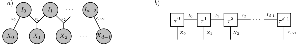
Fig. 7 TT format consisting in the TT hypergraph a) and decorating tensor networks b).
