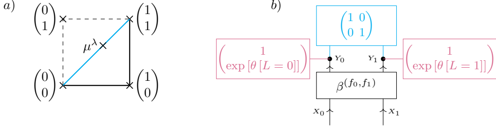
Fig. 5 a) Mean polytope of the statistic t = (X_0 \wedge X_1, X_0 \Rightarrow X_1) (thick), as a subset of the cube [0, 1]^2 (dashed). The blue line is the face of the polytope, which is not cube like, that is not an intersection of the polytope with the faces of the polytope. We further define for \lambda \in (0, 1) a mean parameter \mu_\lambda[L] = [\lambda \lambda]^T which is on the interior of the blue face. b) Corresponding Computation-Activation Network being the maximum entropy distribution reproducing \mu_\lambda[L] , when \lambda is the sigmoid of \theta[L = 0] + \theta[L = 1] .
