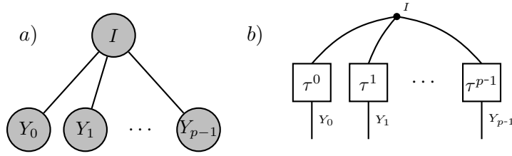
Figure 2: The CP tensor format consist in the CP hypergraph a) and decorating tensor networks b). Tensors in this format constructed as in Lem. 2.10 represent arbitrary faces.
