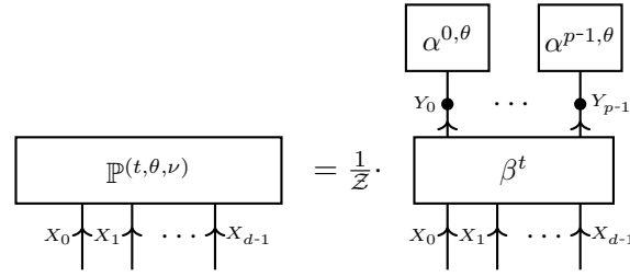
Figure 3: Representation of a member in an exponential family by a Computation-Activation Network with elementary activation. Here Z \in \mathbb{R} is a normalization constant.
