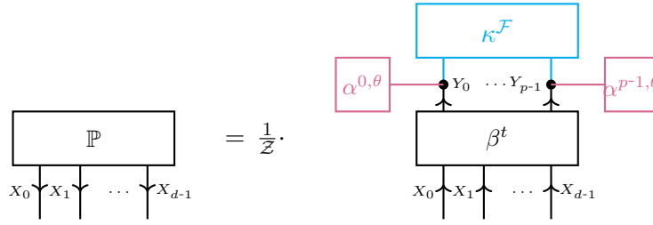
Figure 4: Tensor network decomposition of maximum entropy distributions to the constraint \mu[L] = \langle \mathbb{P}[X_{[d]}], \sigma^t[X_{[d]}, L] \rangle_{[L]} . Blue: Boolean tensor \kappa^{\mathcal{F}}[Y_{[p]}] dependent on the face \mathcal{F}((\mu)) , which represents the refinement of the base measure to the face, and is possibly non-elementary. Red: Elementary activation tensor \alpha^{\theta}[Y_{[p]}] = \bigotimes_{s \in [n]} \alpha^{\ell, \theta}[Y_{\ell}] to the weight \theta[L] = B^{t, \nu^{t, \mathcal{F}}}(\mu) .
