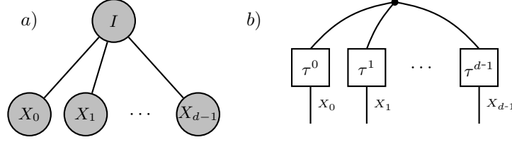
Figure 1: The CP tensor format consist in the CP hypergraph a) and decorating tensor networks b). Tensors in this format constructed as in Lem. 5 represent arbitrary faces.
