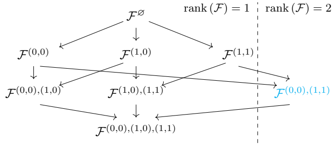
Figure 5: Face lattice L((X_0 \wedge X_1, X_0 \Rightarrow X_1)) to Example 7. The directed arrows represent inclusion of the faces, which is a partial order of the faces. The face \mathcal{F}^{(0,0),(1,1)} is the only face, which is not representable by an elementary hypergraph. It is representable in a CP with hidden rank 2
