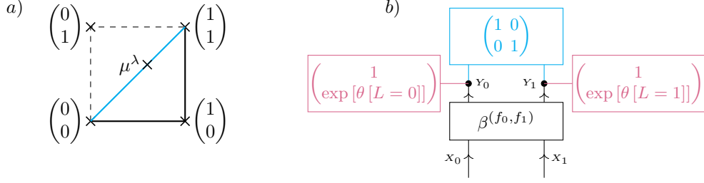
Fig. 4 a) Mean polytope of the statistic t = (X_0 \wedge X_1, X_0 \Rightarrow X_1) (thick), as a subset of the cube [0, 1]^2 (dashed). The blue line is the face of the polytope, which is not cube like, that is not an intersection of the polytope with the faces of the polytope. We further define for \lambda \in (0, 1) a mean parameter \mu_\lambda [L] = [\lambda \ \lambda]^T which is on the interior of the blue face. b) Corresponding Computation-Activation Network being the maximum entropy distribution reproducing \mu_\lambda [L] , when \lambda is the sigmoid of \theta [L = 0] + \theta [L = 1] .
