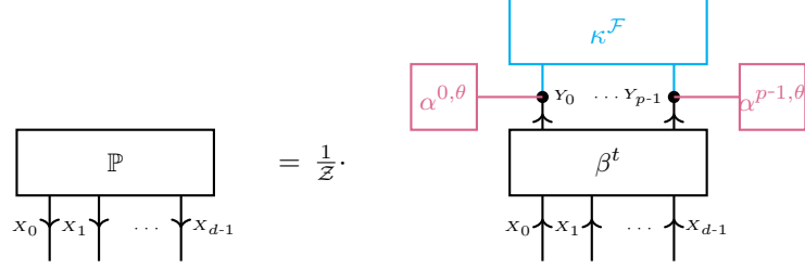
Fig. 3 Tensor network decomposition of maximum entropy distributions to the constraint \mu[L] = \langle \mathbb{P}[X_{[d]}], \sigma^t[X_{[d]}, L] \rangle_{[L]} . Blue: Boolean tensor \kappa^{\mathcal{F}}[Y_{[p]}] dependent on the face \mathcal{F}(\mu) , which represents the refinement of the base measure to the face, and is possibly non-elementary. Red: Elementary activation tensor \alpha^\theta[Y_{[p]}] = \bigotimes_{s \in [n]} \alpha^{\ell, \theta}[Y_\ell] to the weight \theta[L] = B^{t, \nu^t, \mathcal{F}}(\mu) .
