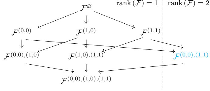
Fig. 5 Face lattice L((X_0 \wedge X_1, X_0 \Rightarrow X_1)) to Example 7. The directed arrows represent inclusion of the faces, which is a partial order of the faces. The face \mathcal{F}^{(0,0),(1,1)} is the only face, which is not representable by an elementary hypergraph. It is representable in a CP with hidden rank 2
