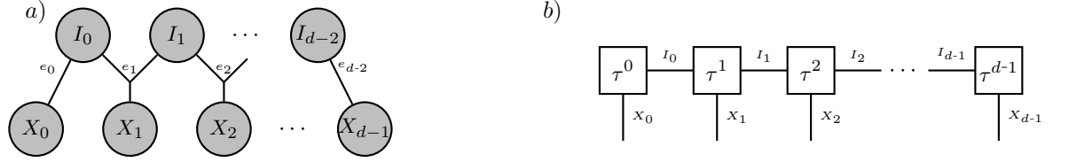
Fig. 6 TT format consisting in the TT hypergraph a) and decorating tensor networks b).
