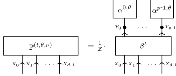
Fig. 2 Representation of a member in an exponential family by a Computation-Activation Network with elementary activation. Here \mathcal{Z} \in \mathbb{R} is a normalization constant.
