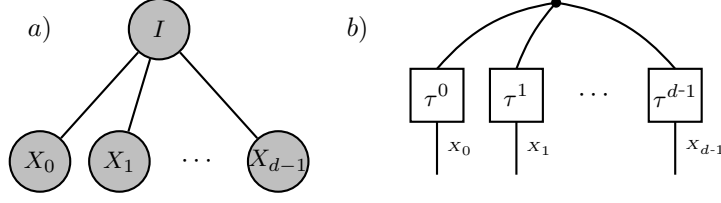
Fig. 1 The CP tensor format consist in the CP hypergraph a) and decorating tensor networks b). Tensors in this format constructed as in Lem. 5 represent arbitrary faces.
